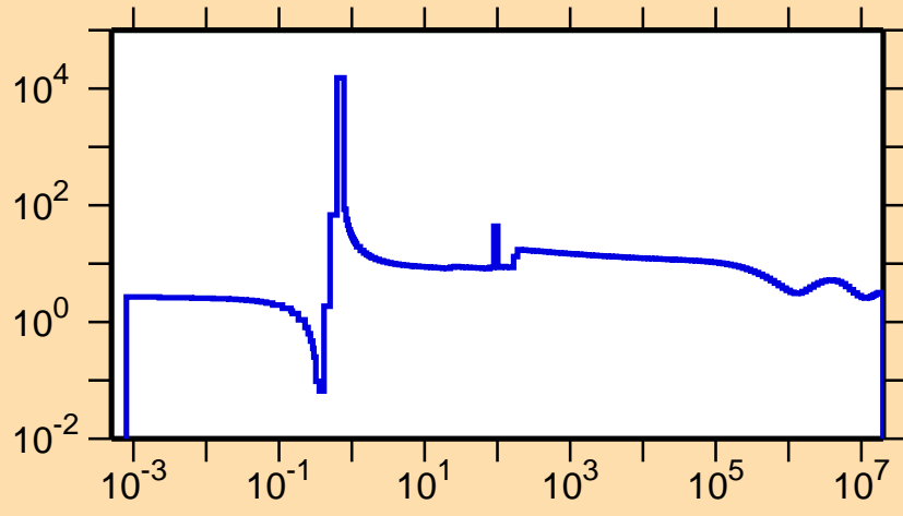
\sigma vs. E for ^{224}\text{Ra}(n,\text{el.})
