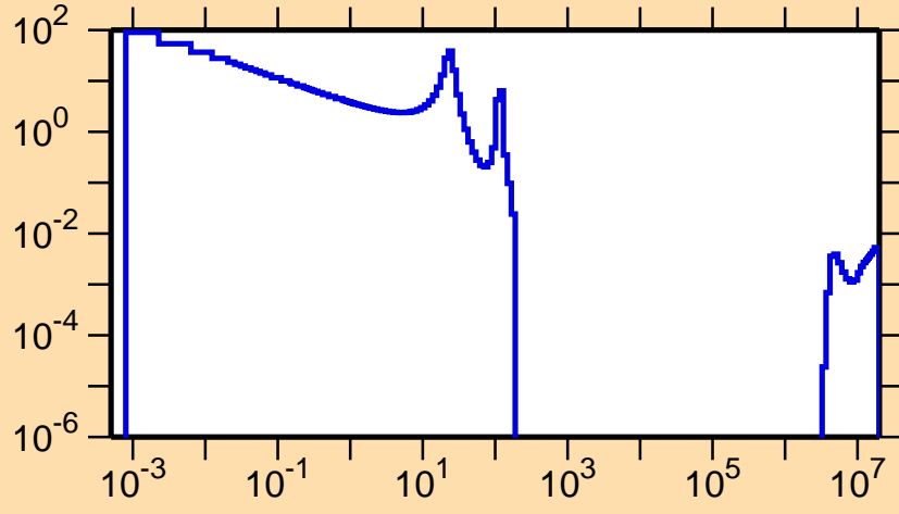
\sigma vs. E for ^{224}\text{Ra}(n,f)
