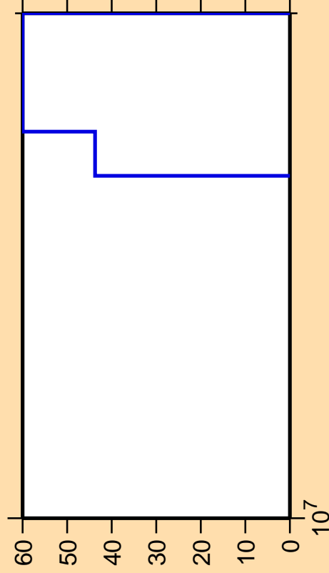
\Delta\sigma/\sigma vs. E for ^{224}\text{Ra} (mt 45)
