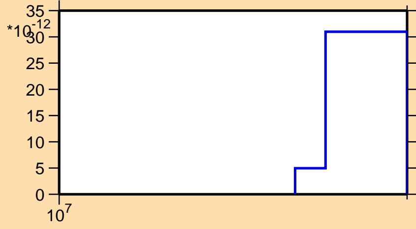
\sigma vs. E for ^{224}\text{Ra} (mt 45)
