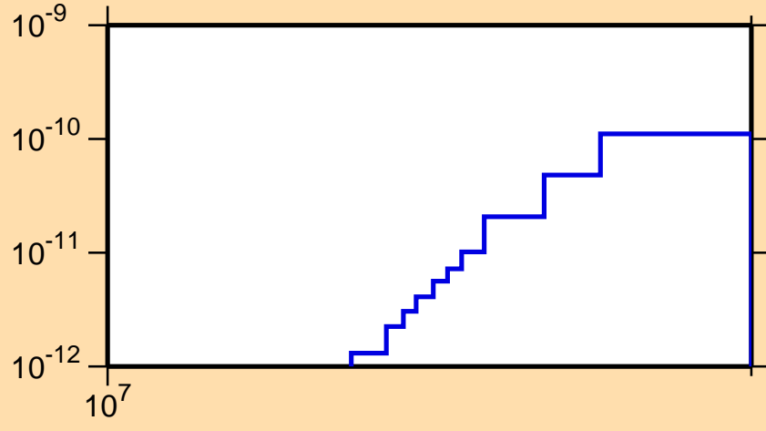
\sigma vs. E for ^{224}\text{Ra}(n,p\alpha)
