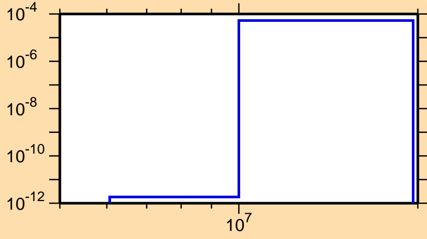
\sigma vs. E for ^{224}\text{Ra}(n,d)
