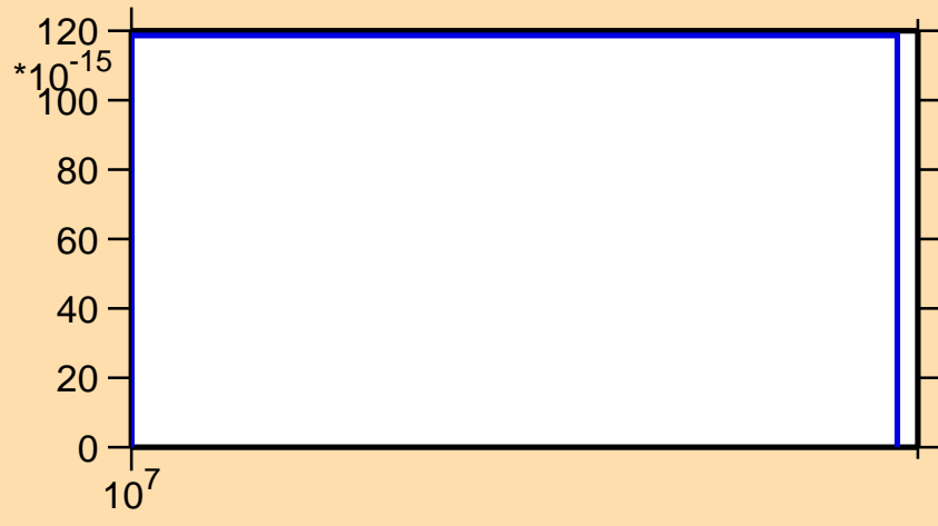
\sigma vs. E for ^{224}\text{Ra}(n,\text{He3})
