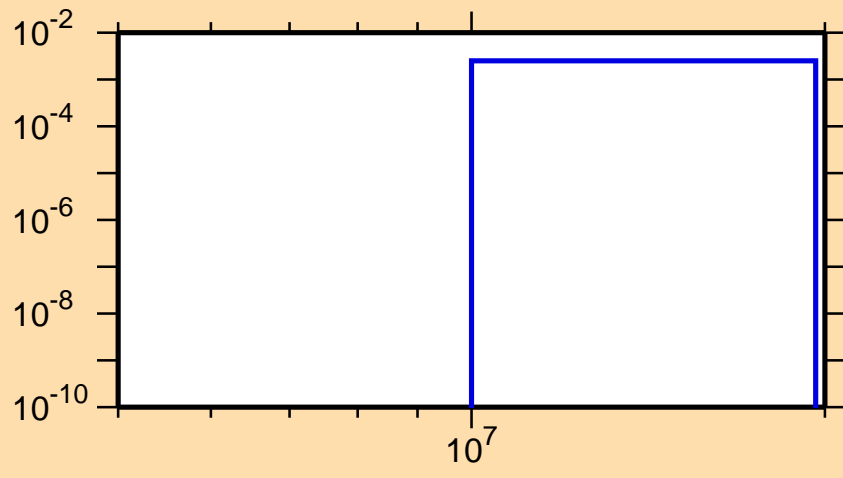
\sigma vs. E for ^{224}\text{Ra}(n,3n\alpha)
