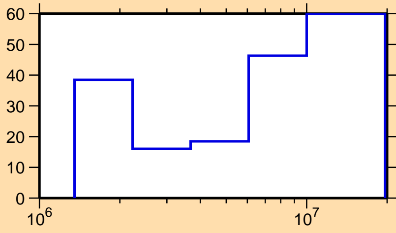
\Delta\sigma/\sigma vs. E for ^{224}\text{Ra}(n,n\text{cont.})
