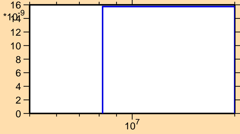
\sigma vs. E for ^{224}\text{Ra}(n,nt)
