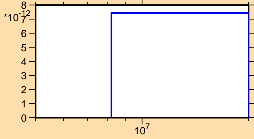
\sigma vs. E for ^{224}\text{Ra}(n,p\alpha)
