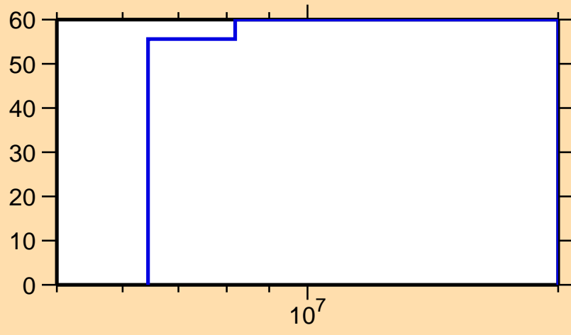
\Delta\sigma/\sigma vs. E for ^{224}\text{Ra}(n,2n)
