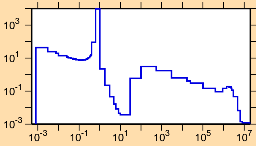
\sigma vs. E for ^{224}\text{Ra}(n,\gamma)
