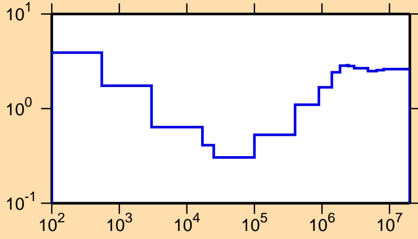
\sigma vs. E for ^{224}\text{Ra}(n,\text{nonel.})
