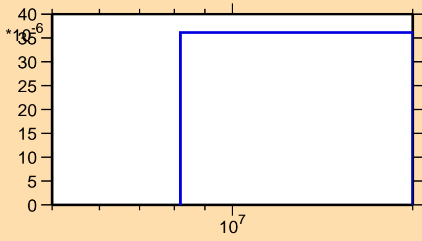
\sigma vs. E for ^{224}\text{Ra}(n,np)
