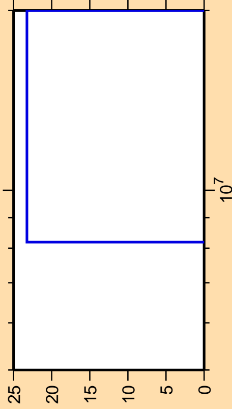
\Delta\sigma/\sigma vs. E for ^{224}\text{Ra}(\text{mt117})
