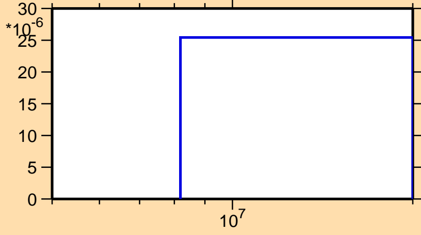
\sigma vs. E for ^{224}\text{Ra}(n,t)
