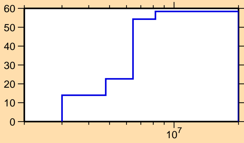
\Delta\sigma/\sigma vs. E for ^{224}\text{Ra}(n,\text{inel.})
