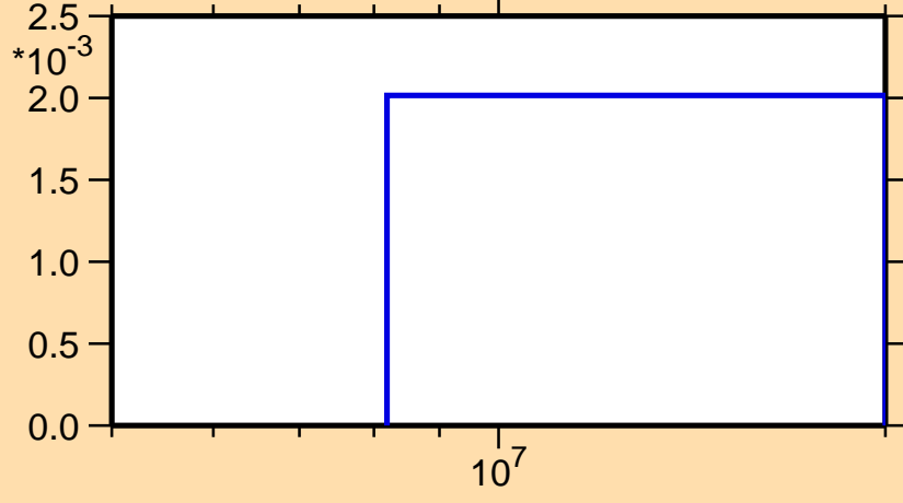
\sigma vs. E for ^{224}\text{Ra}(n,3n\alpha)
