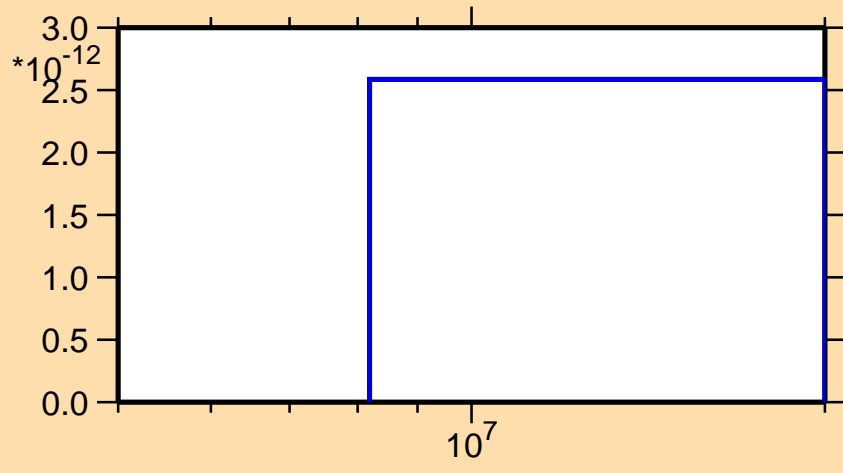
\sigma vs. E for ^{224}\text{Ra}(\text{mt117})
