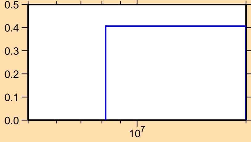
\sigma vs. E for ^{224}\text{Ra}(n,3n)
