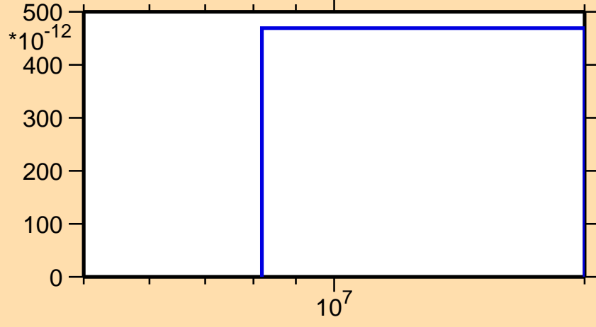
\sigma vs. E for ^{224}\text{Ra}(n,2np)
