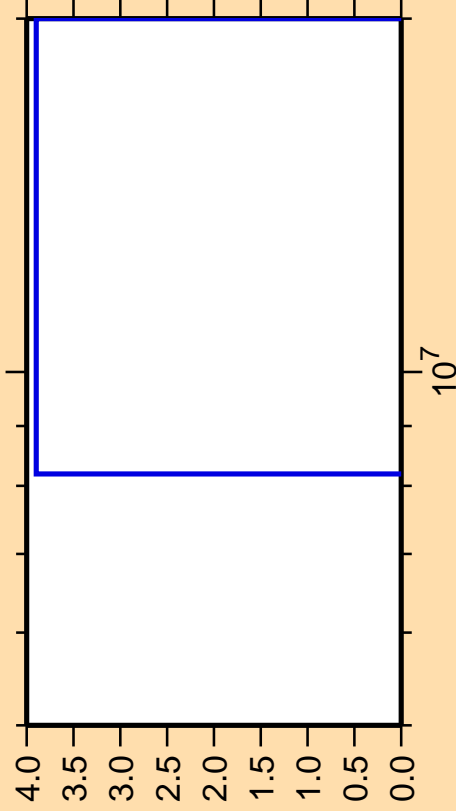
\Delta\sigma/\sigma vs. E for ^{224}\text{Ra}(\text{mt } 45)
