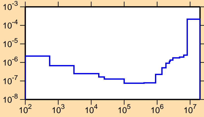
\sigma vs. E for ^{224}\text{Ra}(n,\alpha)
