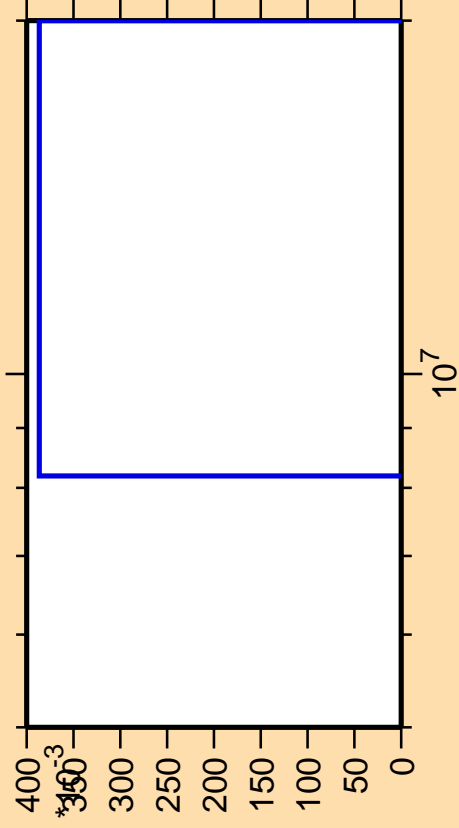
\Delta\sigma/\sigma vs. E for ^{224}\text{Ra}(n,\text{He}3)
