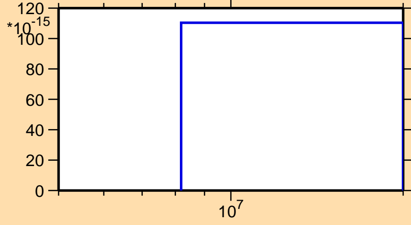
\sigma vs. E for ^{224}\text{Ra}(n,\text{He}3)
