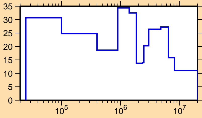
\Delta\sigma/\sigma vs. E for ^{224}\text{Ra}(n,\text{el.})
