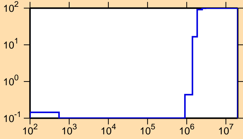
\Delta\sigma/\sigma vs. E for ^{224}\text{Ra}(n,f)
