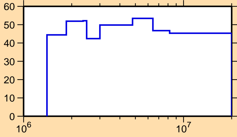
\Delta\sigma/\sigma vs. E for ^{224}\text{Ra}(n,n_1)
