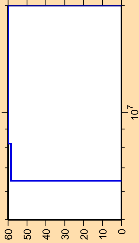
\Delta\sigma/\sigma vs. E for ^{224}\text{Ra}(n,n\text{cont.})
