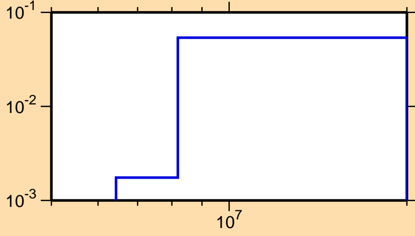
\sigma vs. E for ^{224}\text{Ra}(n,2n\alpha)
