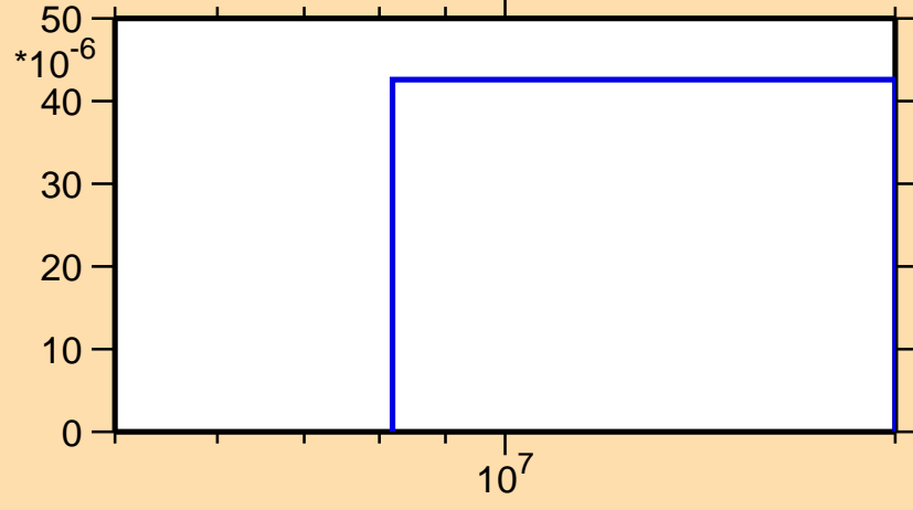
\sigma vs. E for ^{224}\text{Ra}(n,d)
