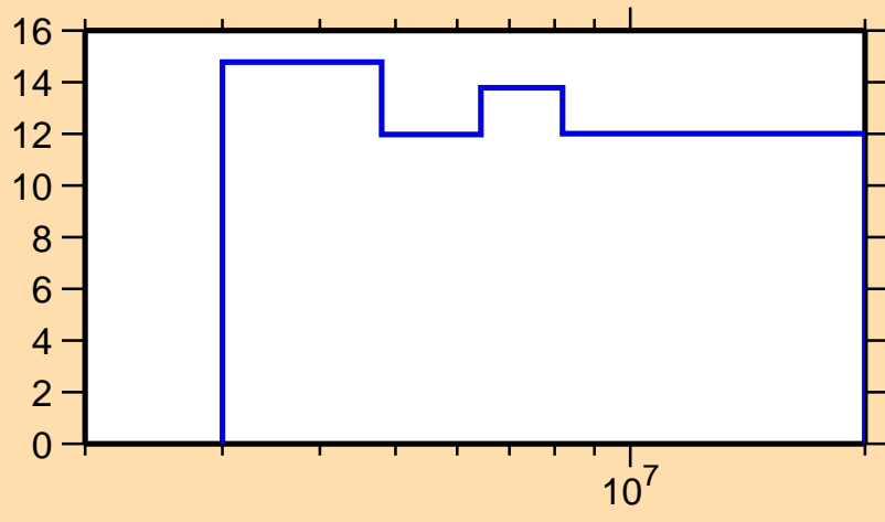
\Delta\sigma/\sigma vs. E for ^{224}\text{Ra}(n,\text{nonel.})
