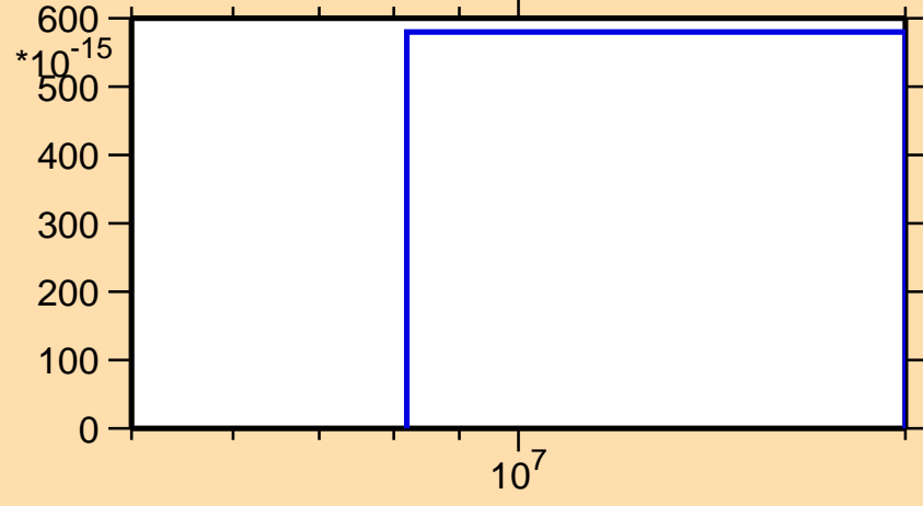
\sigma vs. E for ^{224}\text{Ra}(\text{mt } 45)
