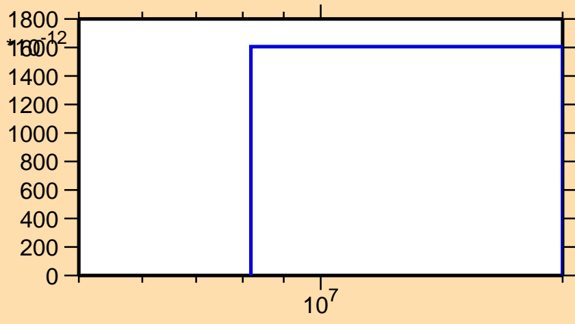
\sigma vs. E for ^{224}\text{Ra}(n,\text{nd})
