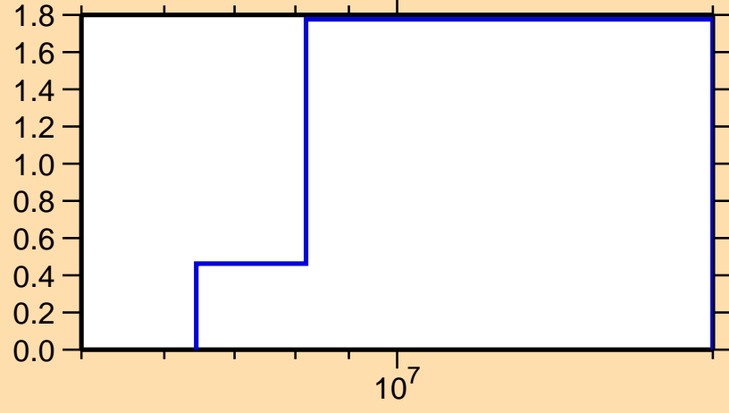
\sigma vs. E for ^{224}\text{Ra}(n,2n)
