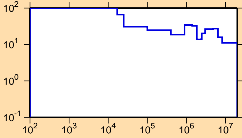
\Delta\sigma/\sigma vs. E for ^{224}\text{Ra}(n,\text{el.})
