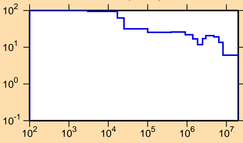
\Delta\sigma/\sigma vs. E for ^{224}\text{Ra}(n,\text{tot.})
