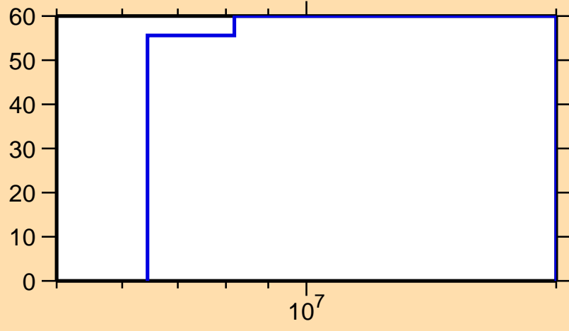
\Delta\sigma/\sigma vs. E for ^{224}\text{Ra}(n,2n)
