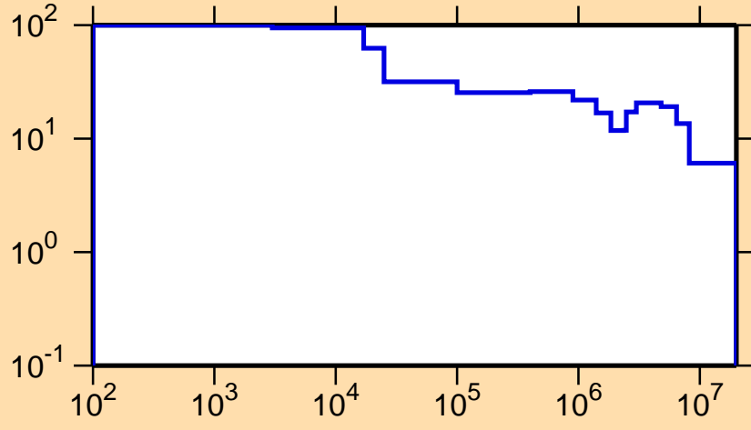
\Delta\sigma/\sigma vs. E for ^{224}\text{Ra}(n,\text{tot.})
