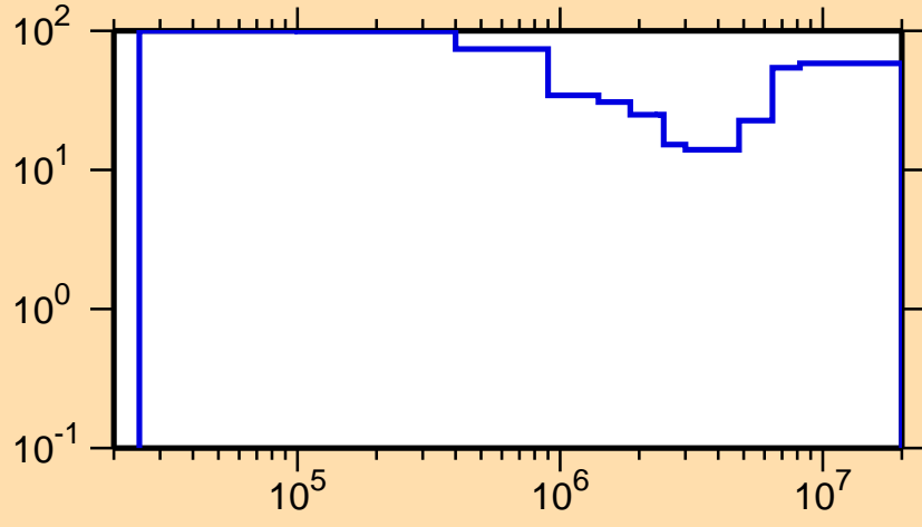
\Delta\sigma/\sigma vs. E for ^{224}\text{Ra}(n,\text{inel.})
