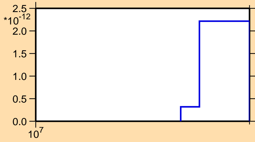
\sigma vs. E for ^{225}\text{Ra}(\text{mt117})
