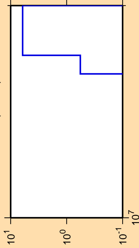
\Delta\sigma/\sigma vs. E for ^{225}\text{Ra} (mt 45)
