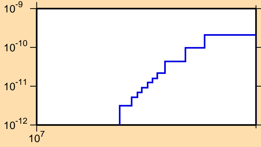
\sigma vs. E for ^{225}\text{Ra}(n,p\alpha)
