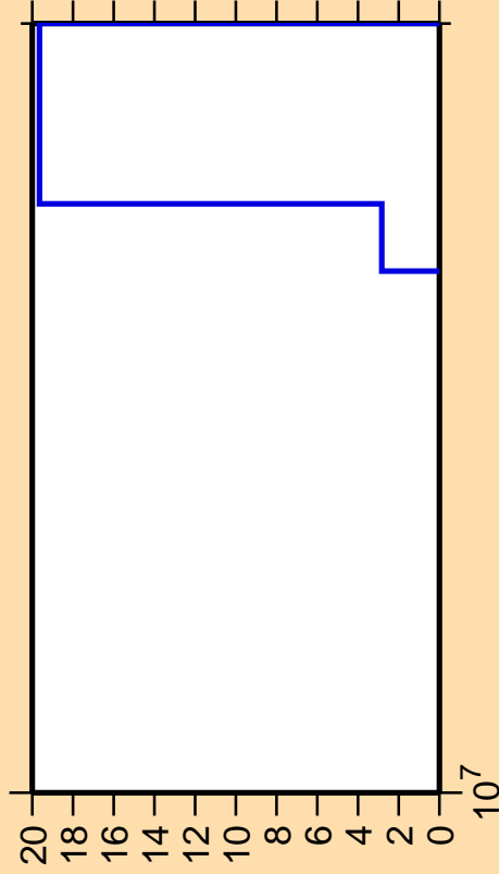
\Delta\sigma/\sigma vs. E for ^{225}\text{Ra}(\text{mt117})
