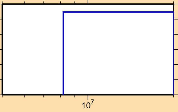
\sigma vs. E for ^{225}\text{Ra}(n,d)
