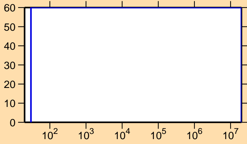
\Delta\sigma/\sigma vs. E for ^{225}\text{Ra}(n,\gamma)
