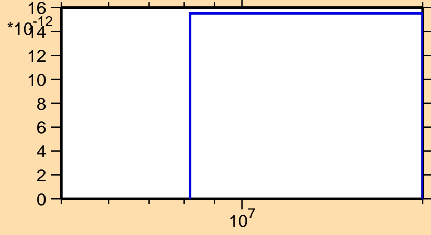
\sigma vs. E for ^{225}\text{Ra}(n,p\alpha)
