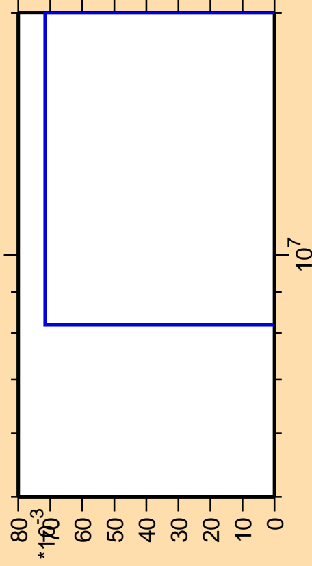
\Delta\sigma/\sigma vs. E for ^{225}\text{Ra} (mt 45)
