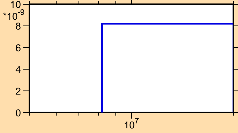
\sigma vs. E for ^{225}\text{Ra}(n,2np)
