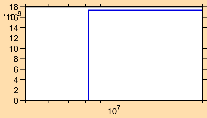
\sigma vs. E for ^{225}\text{Ra}(n,nt)
