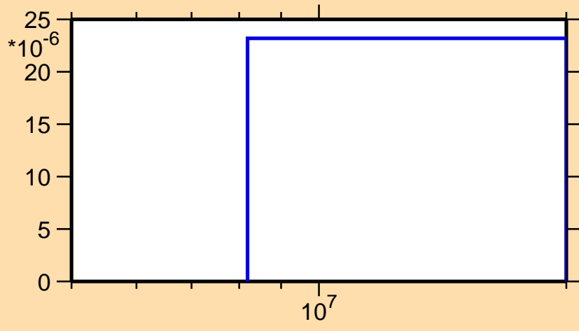
\sigma vs. E for ^{225}\text{Ra}(n,np)
