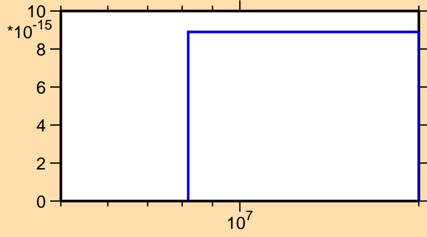
\sigma vs. E for ^{225}\text{Ra} (mt 45)
