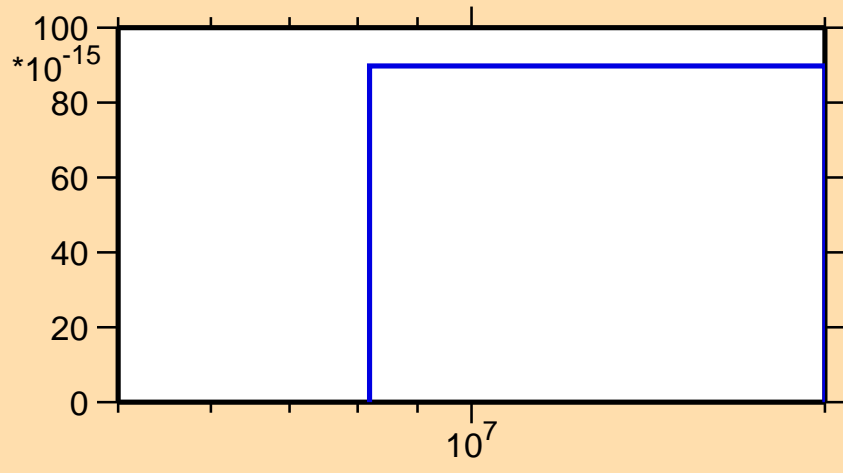
\sigma vs. E for ^{225}\text{Ra}(n,\text{He}3)
