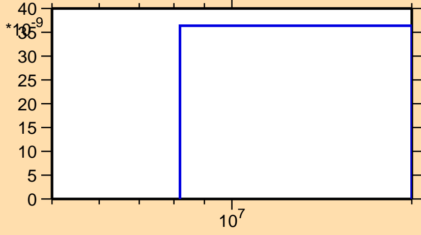
\sigma vs. E for ^{225}\text{Ra}(n,\text{nd})
