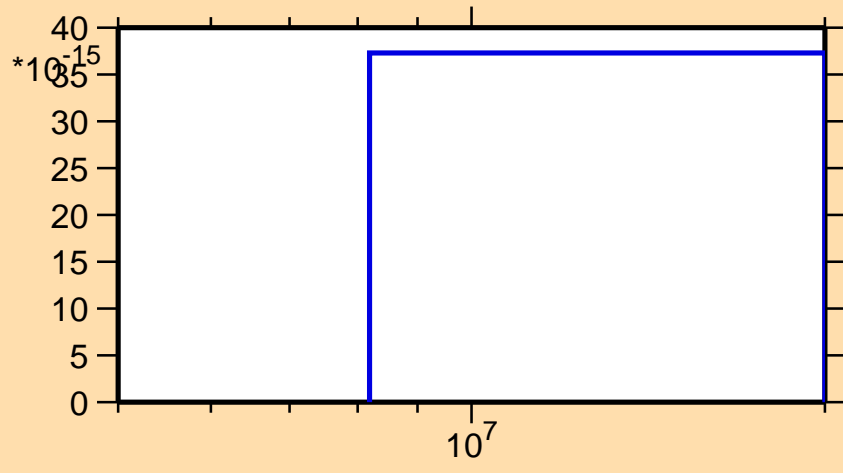
\sigma vs. E for ^{225}\text{Ra}(\text{mt117})
