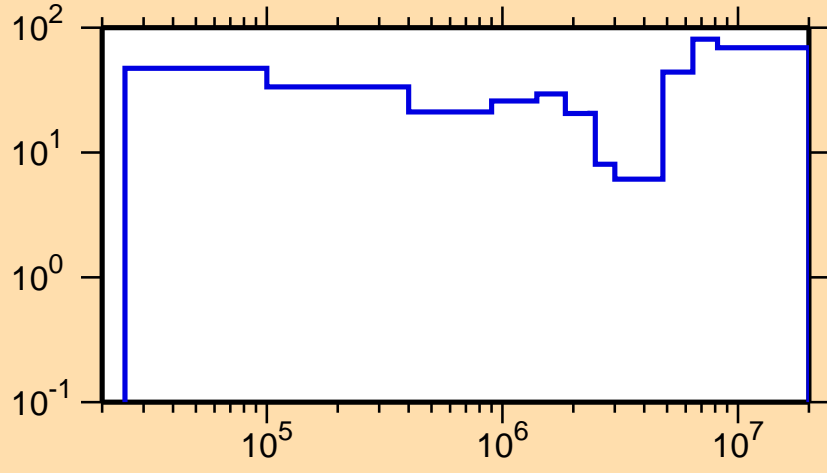
\Delta\sigma/\sigma vs. E for ^{225}\text{Ra}(n,\text{inel.})
