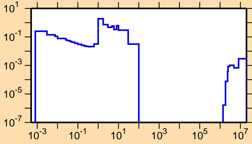
\sigma vs. E for ^{225}\text{Ra}(n,f)
