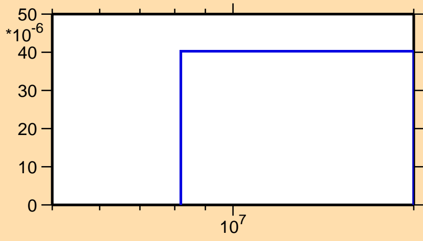
\sigma vs. E for ^{225}\text{Ra}(n,t)
