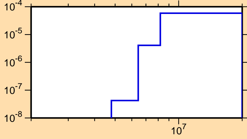
\sigma vs. E for ^{225}\text{Ra}(n,2n\alpha)
