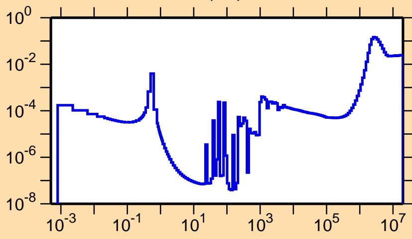
\sigma vs. E for ^{226}\text{Ra}(n,f)
