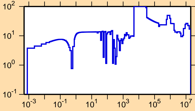
\Delta\sigma/\sigma vs. E for ^{226}\text{Ra}(n,tot.)
