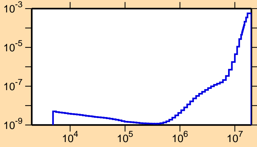
\sigma vs. E for ^{226}\text{Ra}(n,\alpha)
