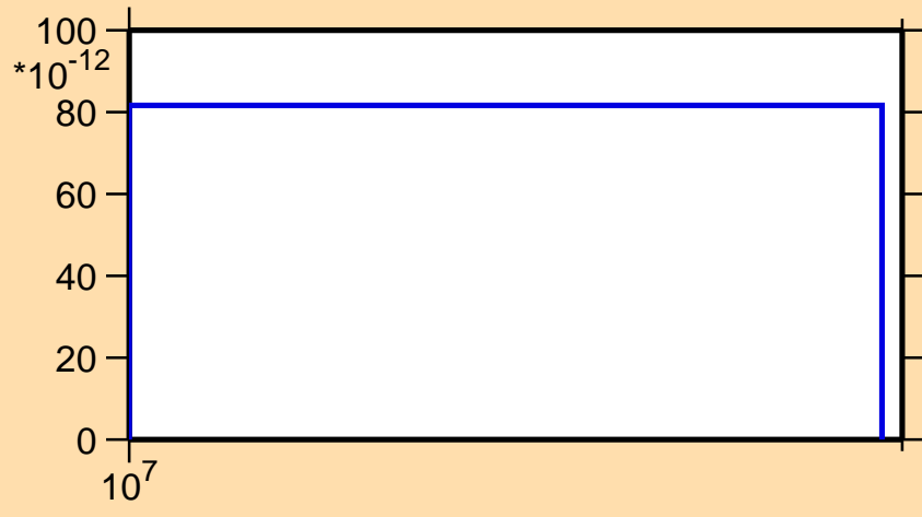
\sigma vs. E for ^{226}\text{Ra}(n,2np)
