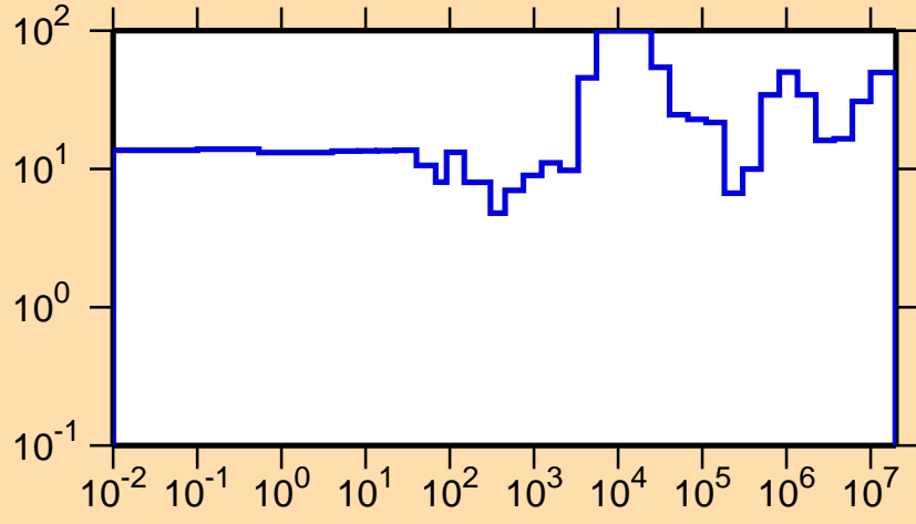
\Delta\sigma/\sigma vs. E for ^{226}\text{Ra}(n,el.)
