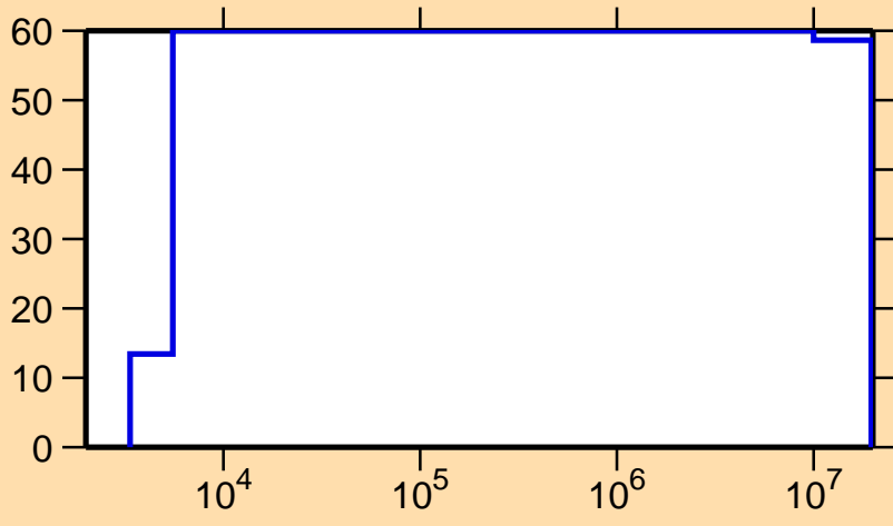
\Delta\sigma/\sigma vs. E for ^{226}\text{Ra}(n,\gamma)
