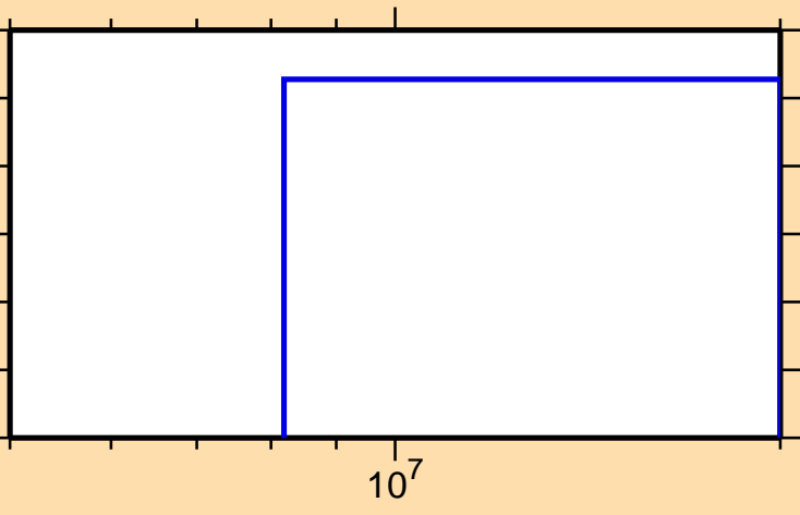
\sigma vs. E for ^{226}\text{Ra}(n,\text{nd})
