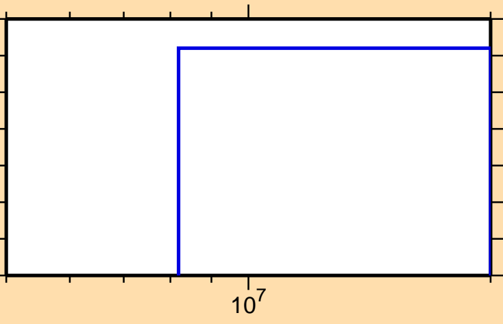
\sigma vs. E for ^{226}\text{Ra}(n,np)
