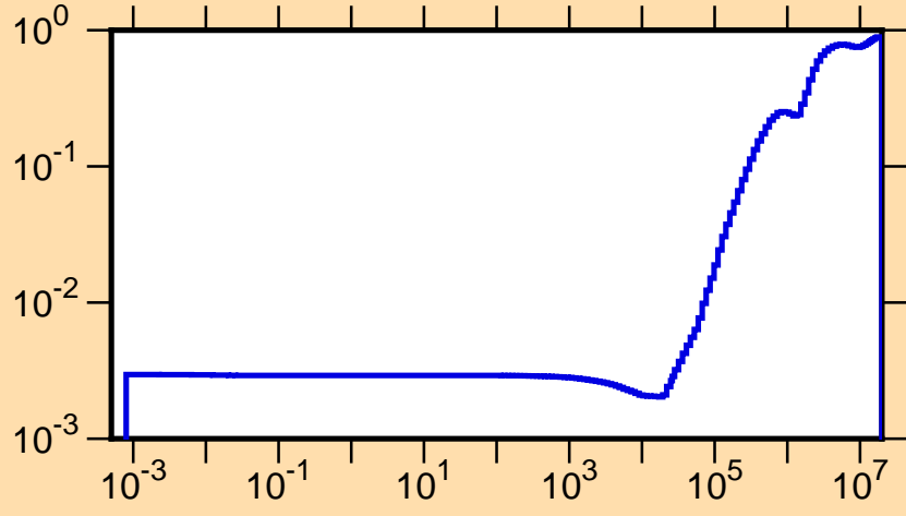
\mu vs. E for ^{227}\text{Ra}(\text{mt251})
