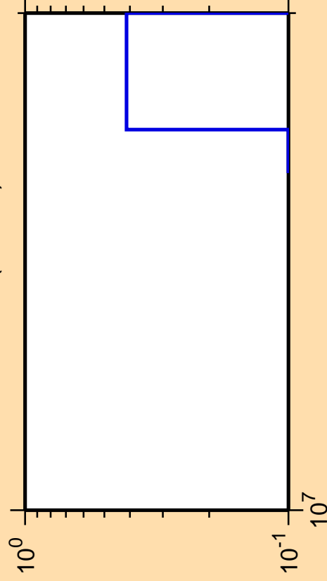
\Delta\sigma/\sigma vs. E for ^{227}\text{Ra}(n,\text{He}3)
