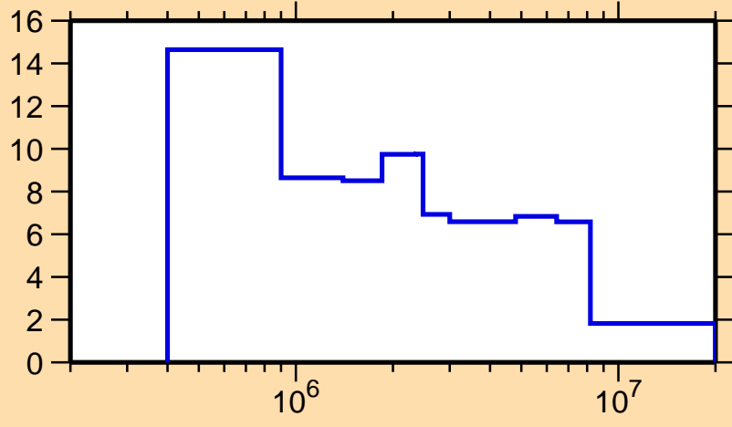
\Delta\sigma/\sigma vs. E for ^{227}\text{Ra}(n, el.)
