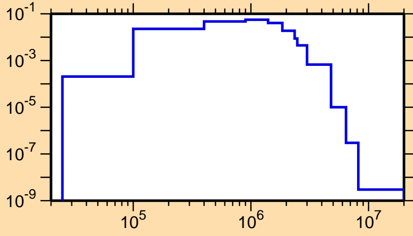
\sigma vs. E for ^{227}\text{Ra}(n,n_4)
