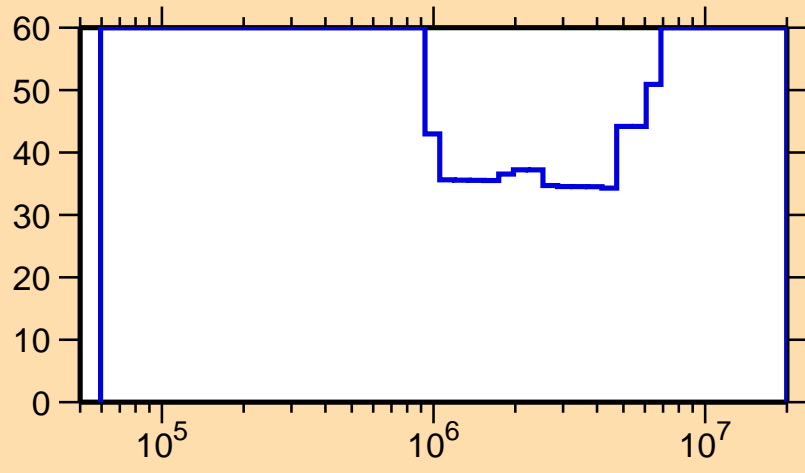
\Delta\sigma/\sigma vs. E for ^{228}\text{Ra}(n,\text{inel.})
