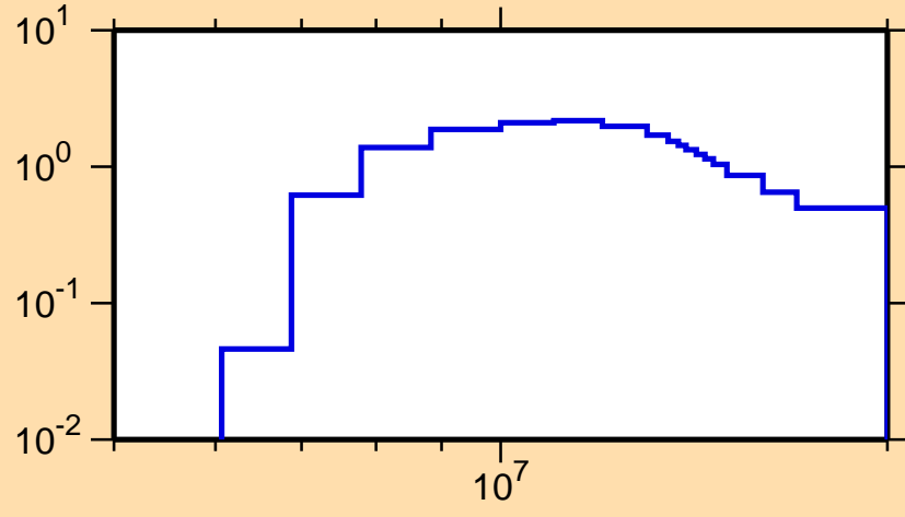
\sigma vs. E for ^{228}\text{Ra}(n,2n)
