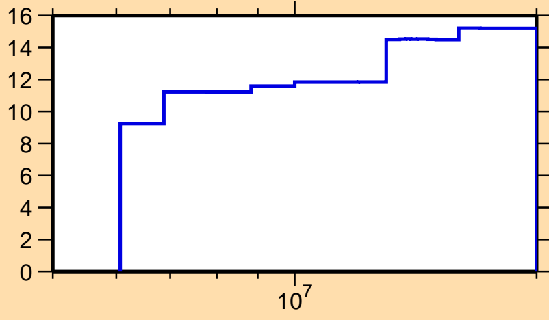
\Delta\sigma/\sigma vs. E for ^{228}\text{Ra}(n,\text{nonel.})
