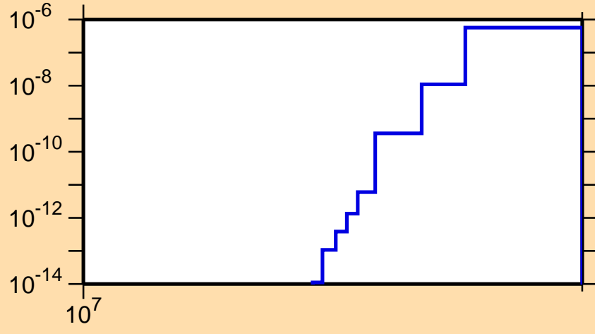
\sigma vs. E for ^{228}\text{Ra}(n,nt)
