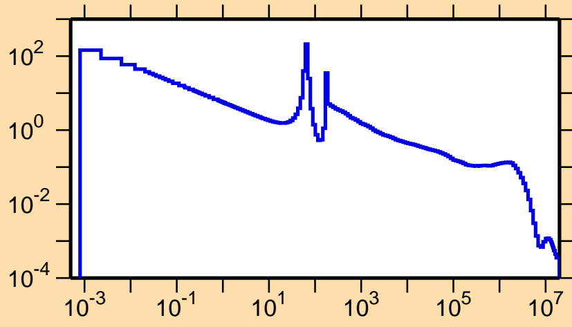
\sigma vs. E for ^{228}\text{Ra}(n,\gamma)
