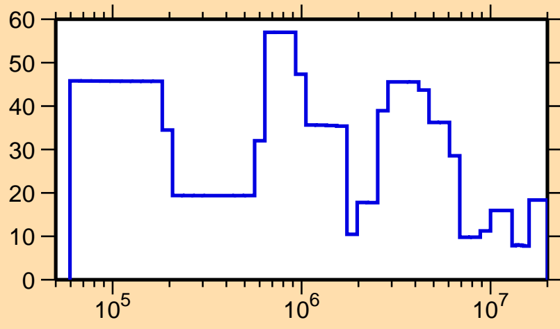
\Delta\sigma/\sigma vs. E for ^{228}\text{Ra}(n,\text{el.})
