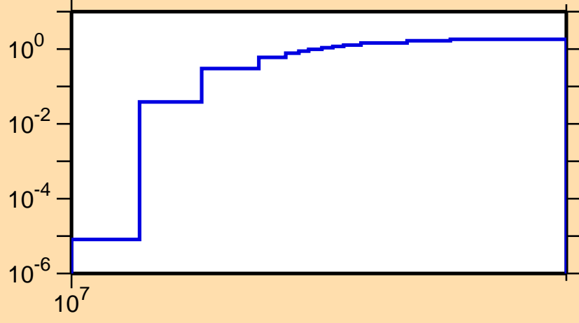
\sigma vs. E for ^{228}\text{Ra}(n,3n)
