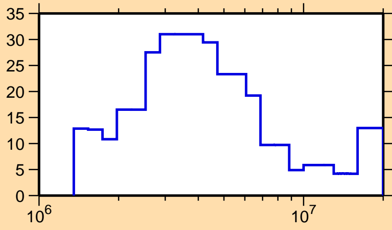
\Delta\sigma/\sigma vs. E for ^{228}\text{Ra}(n,\text{tot.})
