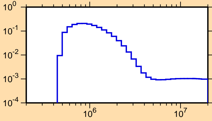
\sigma vs. E for ^{228}\text{Ra}(n,n_4)
