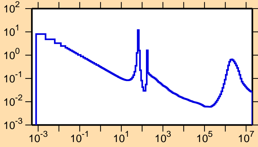
\sigma vs. E for ^{228}\text{Ra}(n,f)
