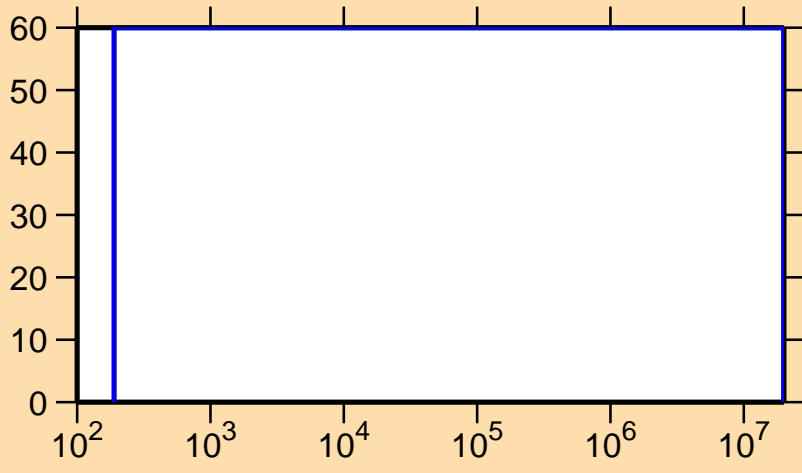
\Delta\sigma/\sigma vs. E for ^{228}\text{Ra}(n,\gamma)
