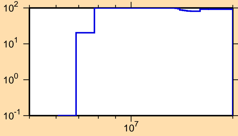
\Delta\sigma/\sigma vs. E for ^{228}\text{Ra}(n,p)
