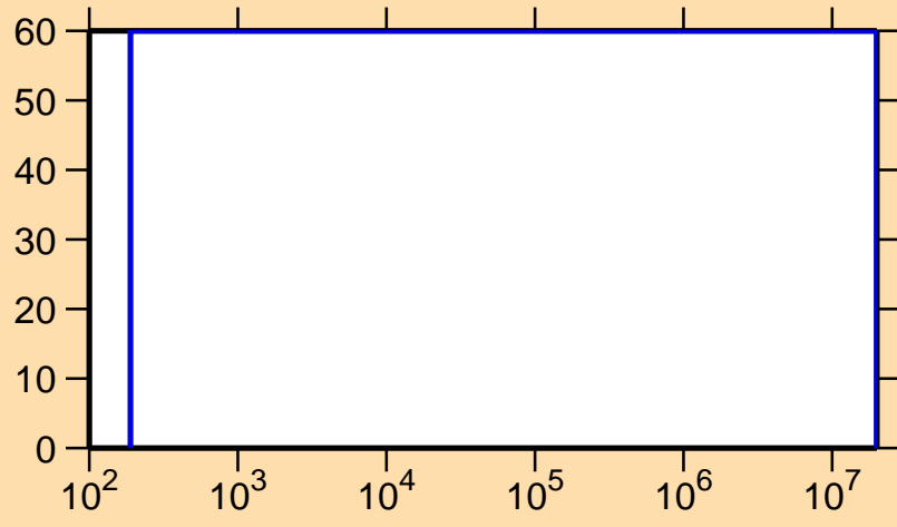
\Delta\sigma/\sigma vs. E for ^{228}\text{Ra}(n,f)
