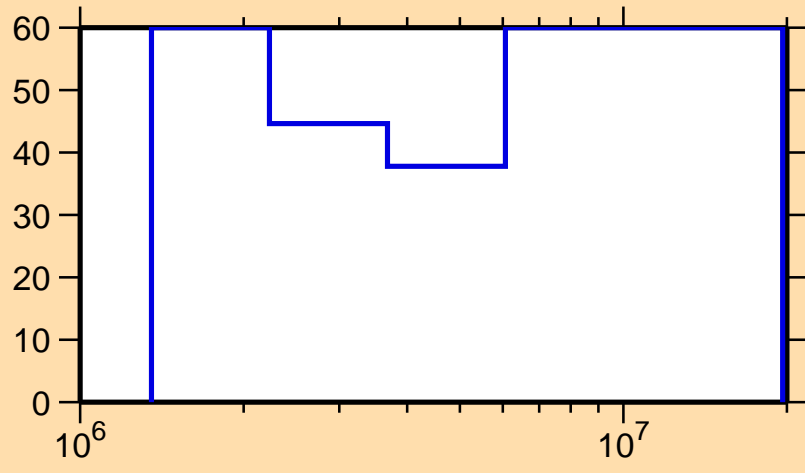
\Delta\sigma/\sigma vs. E for ^{228}\text{Ra}(n,n\text{cont.})
