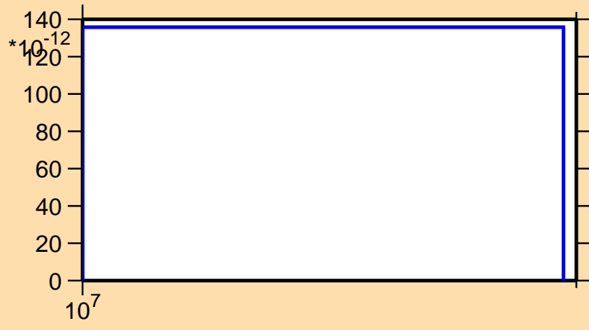
\sigma vs. E for ^{228}\text{Ra}(n,\text{nd})
