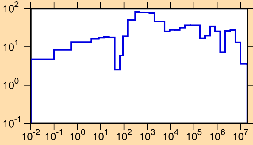
\Delta\sigma/\sigma vs. E for ^{228}\text{Ra}(n,tot.)
