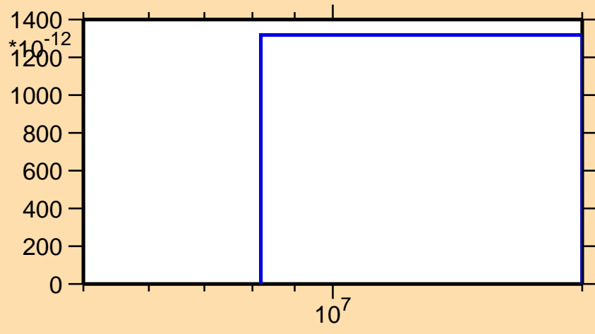
\sigma vs. E for ^{228}\text{Ra}(n,3n\alpha)
