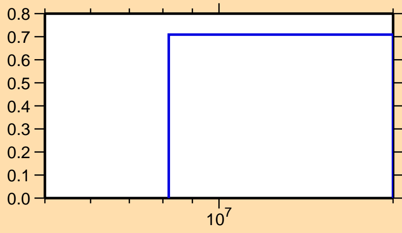
\sigma vs. E for ^{228}\text{Ra}(n,3n)
