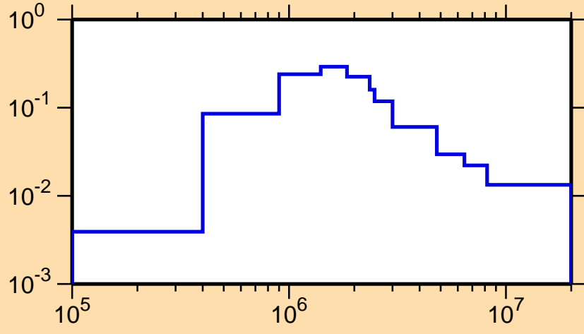
\sigma vs. E for ^{228}\text{Ra}(n,n_2)
