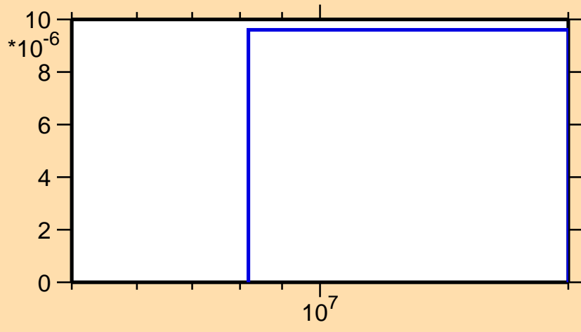
\sigma vs. E for ^{228}\text{Ra}(n,d)
