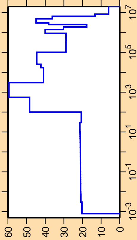
\Delta\sigma/\sigma vs. E for ^{228}\text{Ra}(n,\text{el.})
