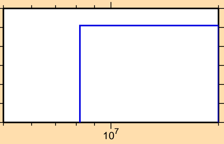
\sigma vs. E for ^{228}\text{Ra}(n,nt)
