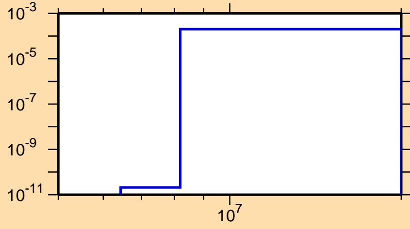
\sigma vs. E for ^{228}\text{Ra}(n,p)
