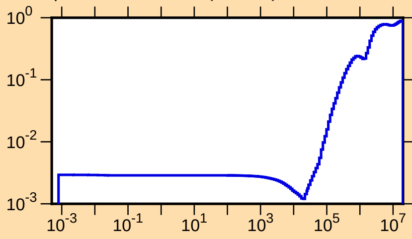
\mu vs. E for ^{229}\text{Ra}(\text{mt251})
