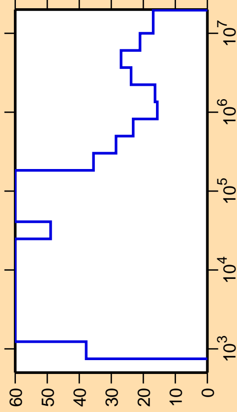
\Delta\sigma/\sigma vs. E for ^{230}\text{Ra}(n,\text{nonel.})
