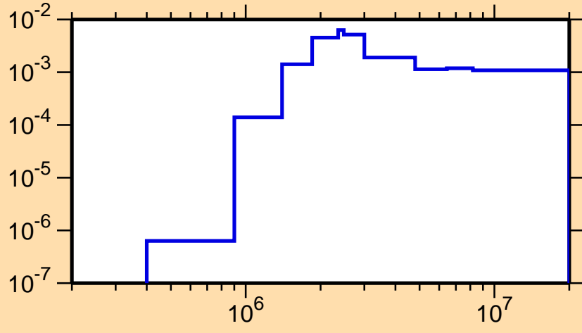
\sigma vs. E for ^{230}\text{Ra}(n,n_4)
