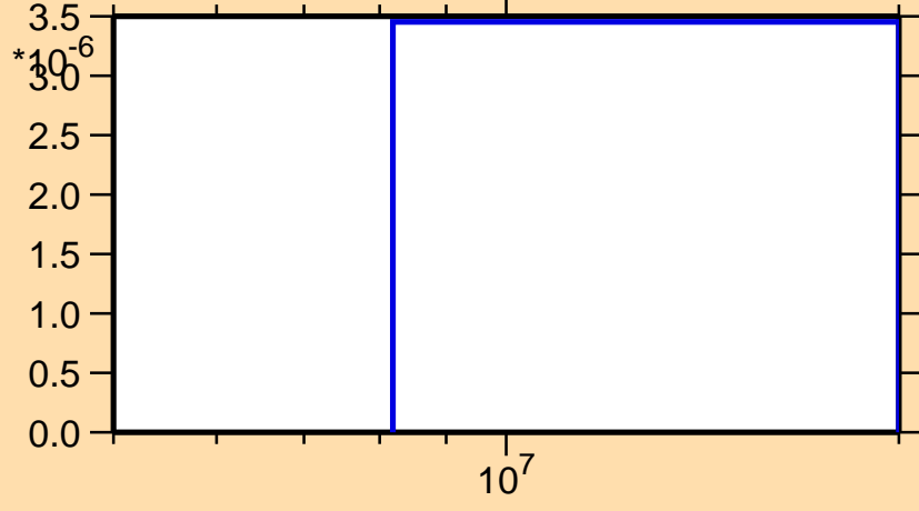
\sigma vs. E for ^{230}\text{Ra}(n,t)
