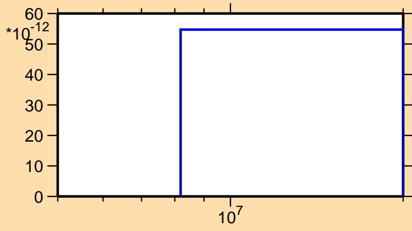
\sigma vs. E for ^{230}\text{Ra}(n,3n\alpha)
