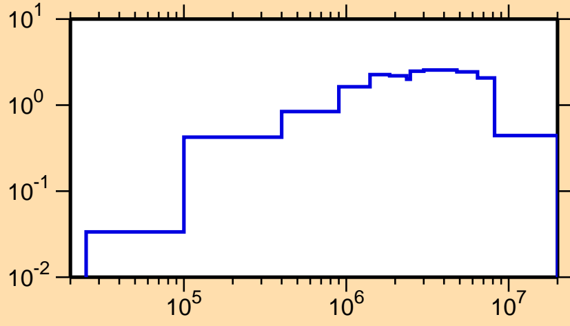
\sigma vs. E for ^{230}\text{Ra}(n,\text{inel.})
