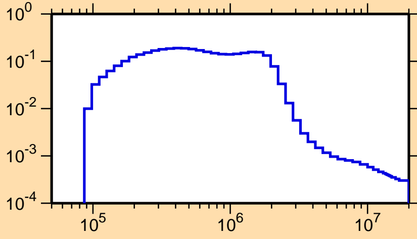
\sigma vs. E for ^{231}\text{Ra}(n,n_3)
