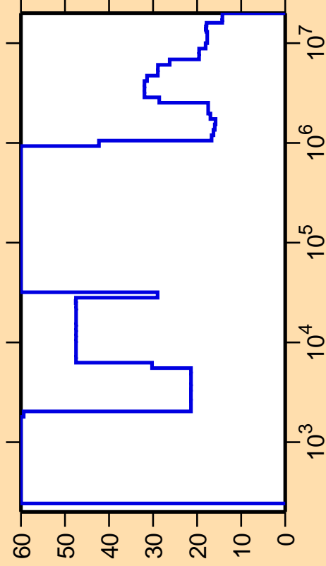
\Delta\sigma/\sigma vs. E for ^{231}\text{Ra}(n,\text{nonel.})
