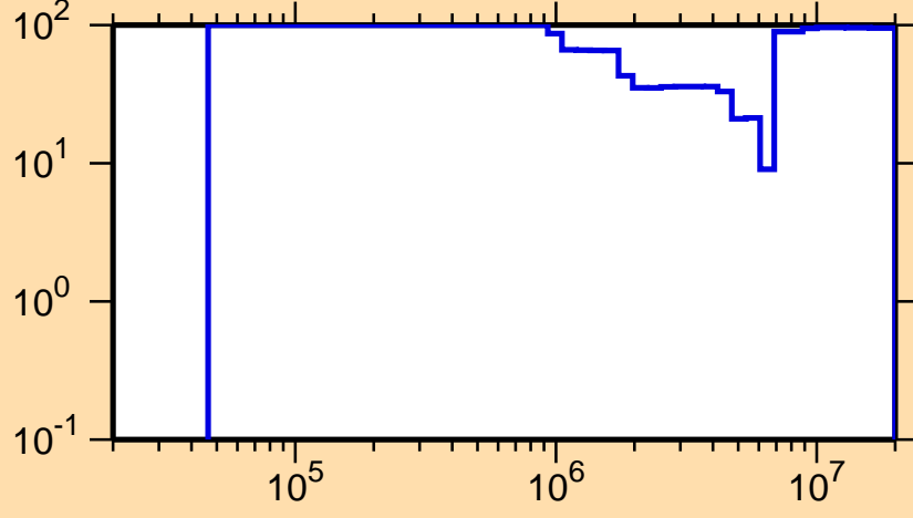
\Delta\sigma/\sigma vs. E for ^{231}\text{Ra}(n,\text{inel.})
