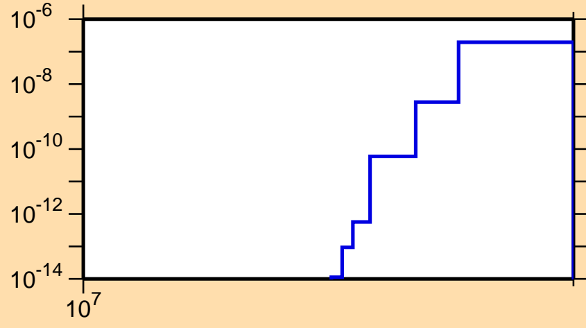
\sigma vs. E for ^{231}\text{Ra}(n,\text{nd})
