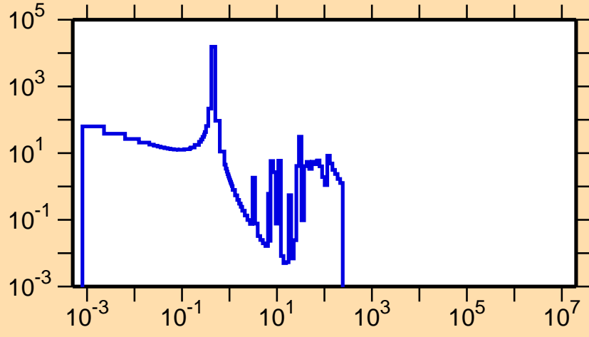
\sigma vs. E for ^{231}\text{Ra}(n,f)
