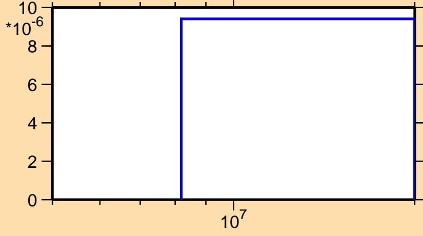
\sigma vs. E for ^{231}\text{Ra}(n,t)
