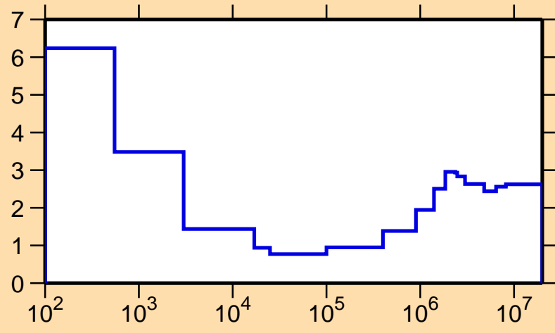
\sigma vs. E for ^{231}\text{Ra}(n,\text{nonel.})
