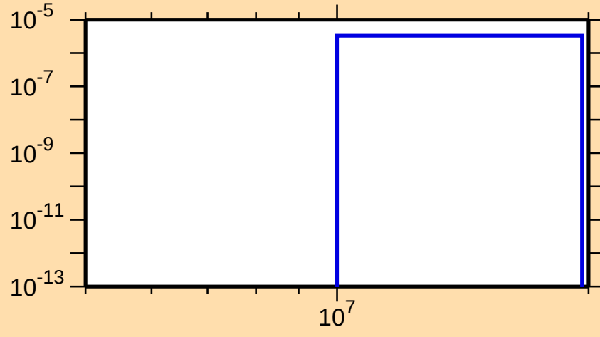
\sigma vs. E for ^{232}\text{Ra}(n,t)
