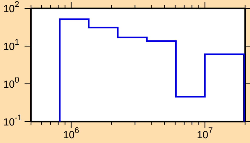
\Delta\sigma/\sigma vs. E for ^{232}\text{Ra}(n,\text{nonel.})
