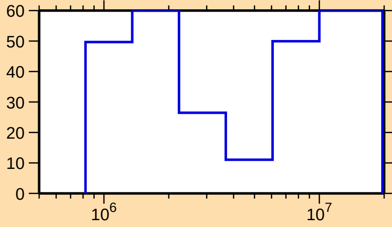
\Delta\sigma/\sigma vs. E for ^{232}\text{Ra}(n,\text{tot.})
