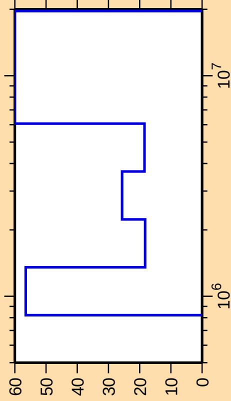
\Delta\sigma/\sigma vs. E for ^{232}\text{Ra}(n,n\text{cont.})
