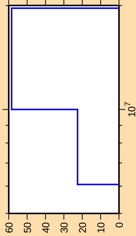
\Delta\sigma/\sigma vs. E for ^{232}\text{Ra}(n,p)
