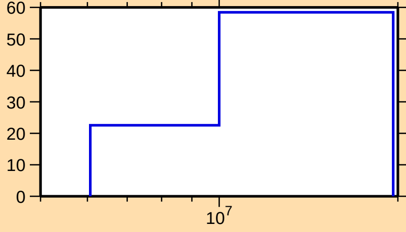
\Delta\sigma/\sigma vs. E for ^{232}\text{Ra}(n,p)
