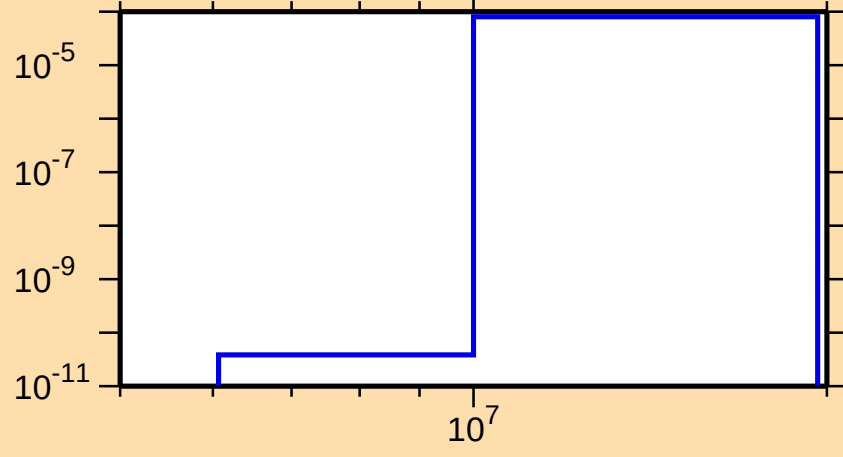
\sigma vs. E for ^{232}\text{Ra}(n,p)
