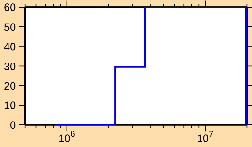
\Delta\sigma/\sigma vs. E for ^{232}\text{Ra}(n,f)
