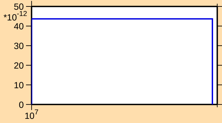
\sigma vs. E for ^{232}\text{Ra}(n,\text{nd})
