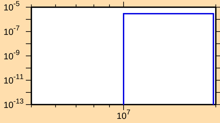
\sigma vs. E for ^{232}\text{Ra}(n,d)
