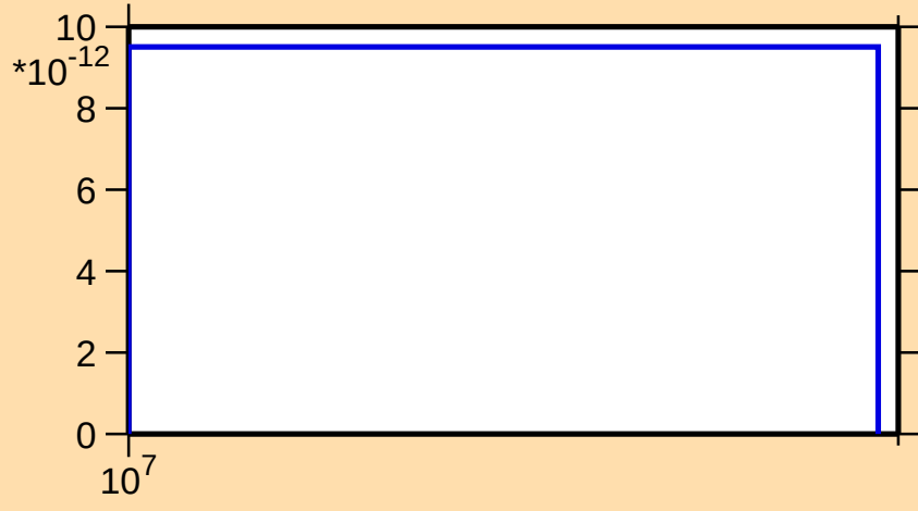
\sigma vs. E for ^{232}\text{Ra}(n,3n\alpha)
