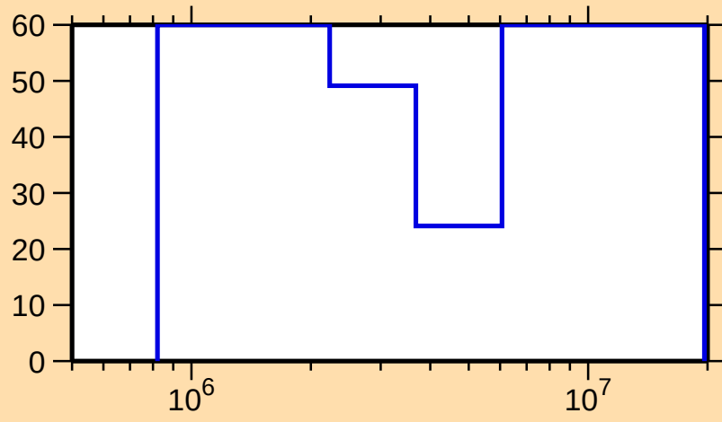
\Delta\sigma/\sigma vs. E for ^{232}\text{Ra}(n,\text{el.})
