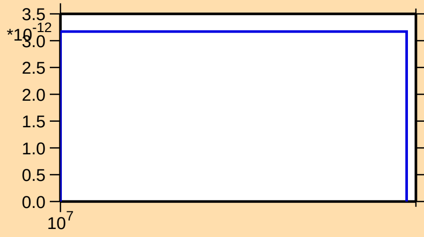
\sigma vs. E for ^{232}\text{Ra}(n,2np)
