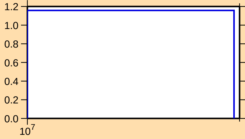
\sigma vs. E for ^{232}\text{Ra}(n,3n)
