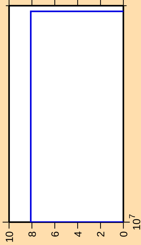
\Delta\sigma/\sigma vs. E for ^{232}\text{Ra}(n,3n\alpha)
