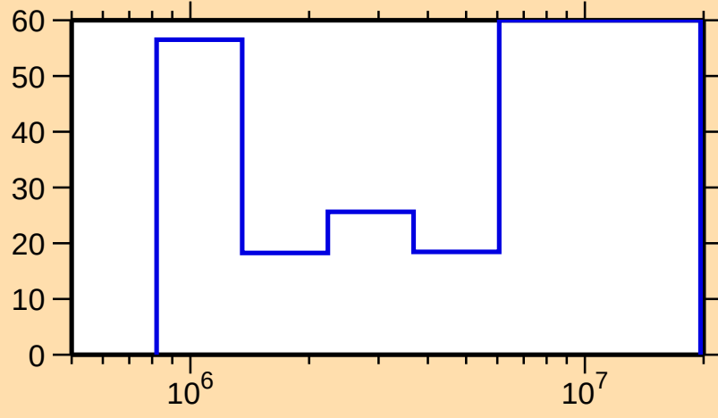
\Delta\sigma/\sigma vs. E for ^{232}\text{Ra}(n,n\text{cont.})
