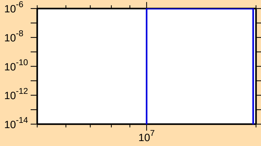
\sigma vs. E for ^{232}\text{Ra}(n,np)
