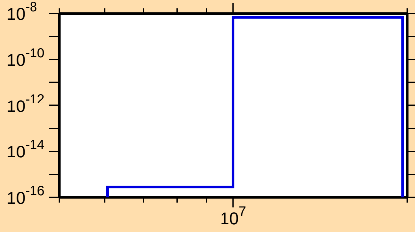
\sigma vs. E for ^{232}\text{Ra}(n,2n\alpha)
