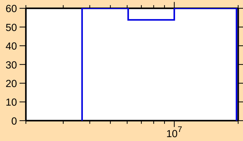
\Delta\sigma/\sigma vs. E for ^{232}\text{Ra}(n,2n)
