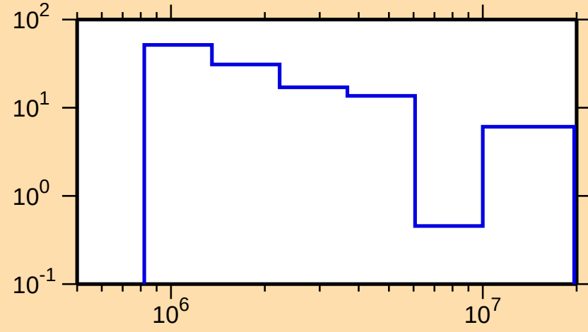
\Delta\sigma/\sigma vs. E for ^{232}\text{Ra}(n,n\text{onel.})
