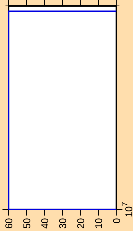
\Delta\sigma/\sigma vs. E for ^{232}\text{Ra}(n,\text{nt})
