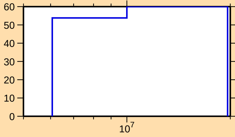
\Delta\sigma/\sigma vs. E for ^{232}\text{Ra}(n,2n)
