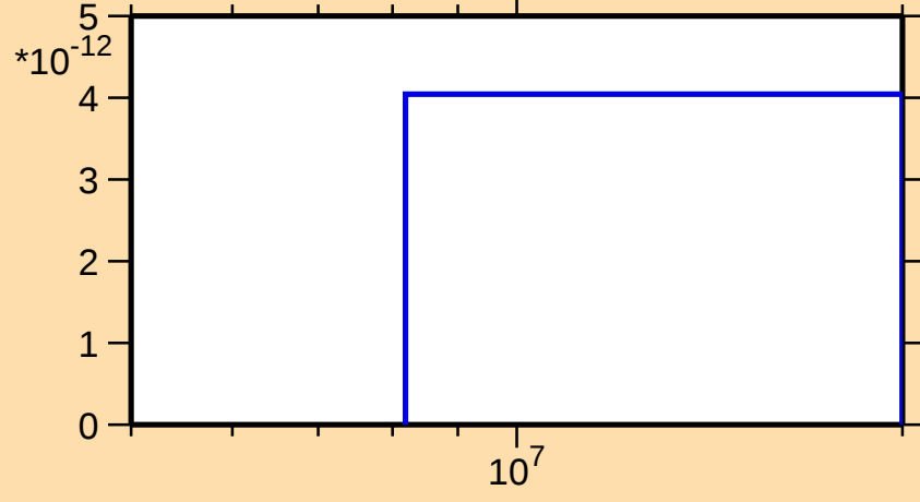
\sigma vs. E for ^{232}\text{Ra}(n,2np)
