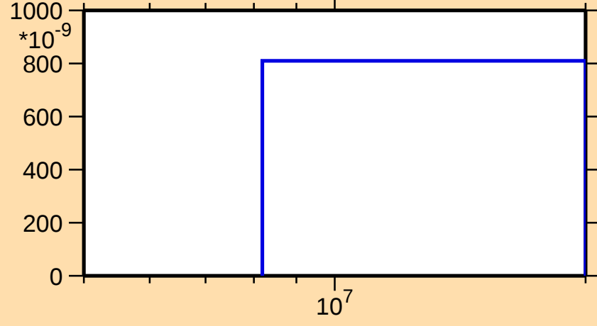
\sigma vs. E for ^{232}\text{Ra}(n,np)
