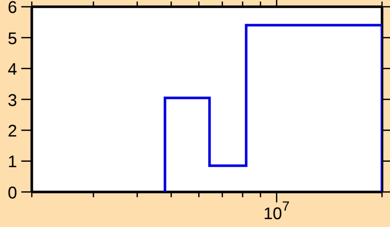
\Delta\sigma/\sigma vs. E for ^{232}\text{Ra}(n,\text{nonel.})
