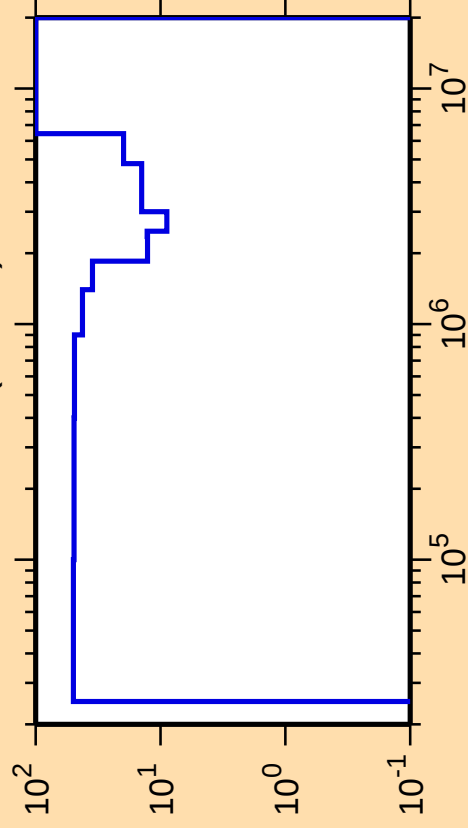
\Delta\sigma/\sigma vs. E for ^{232}\text{Ra}(n,\text{inel.})
