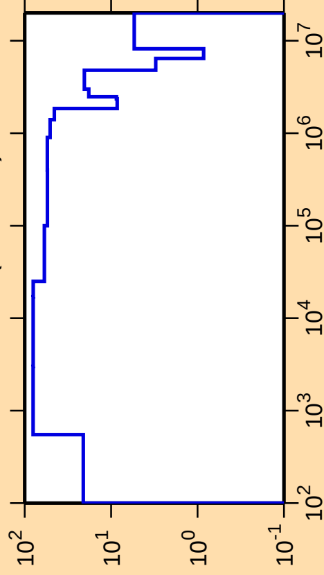
\Delta\sigma/\sigma vs. E for ^{232}\text{Ra}(n,\text{nonel.})
