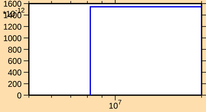
\sigma vs. E for ^{232}\text{Ra}(n,nt)
