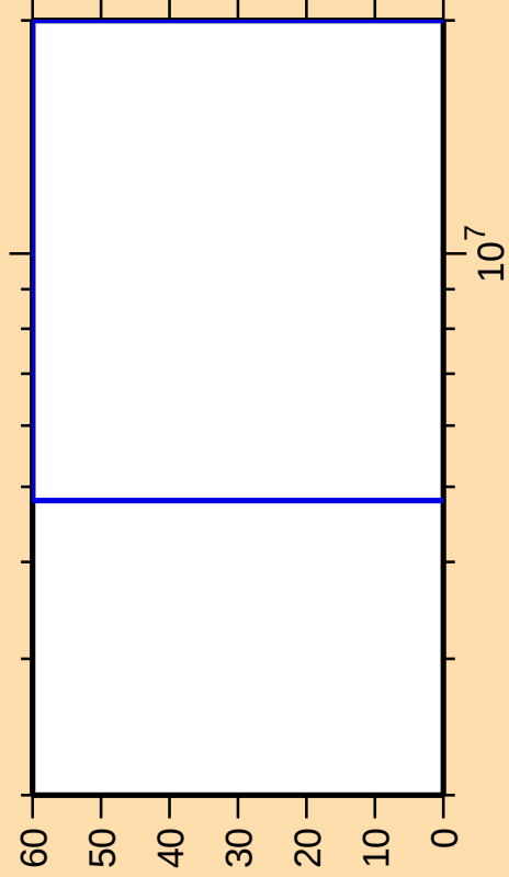
\Delta\sigma/\sigma vs. E for ^{232}\text{Ra}(n,2n)
