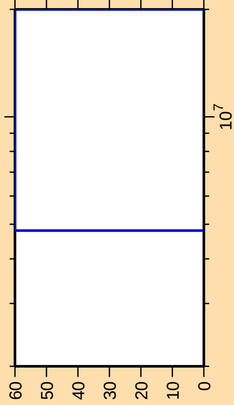
\Delta\sigma/\sigma vs. E for ^{232}\text{Ra}(n,f)
