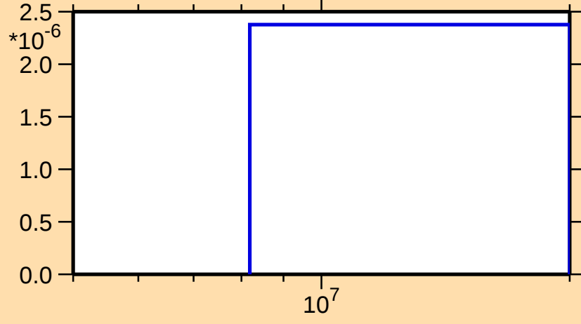
\sigma vs. E for ^{232}\text{Ra}(n,d)
