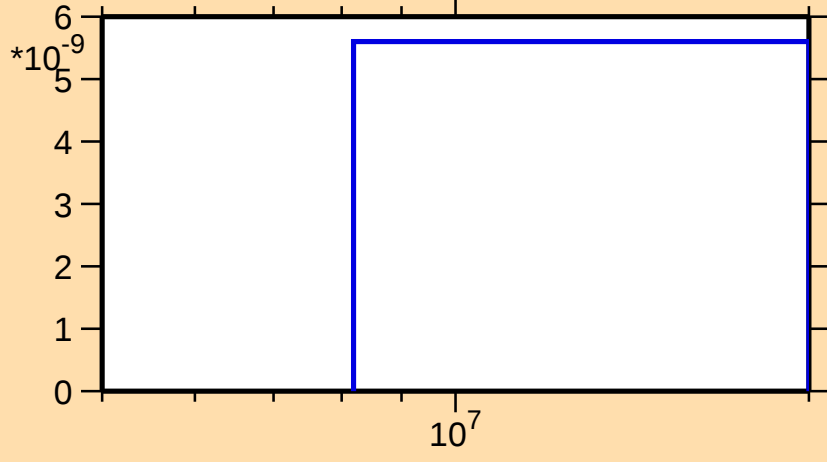
\sigma vs. E for ^{232}\text{Ra}(n,2n\alpha)
