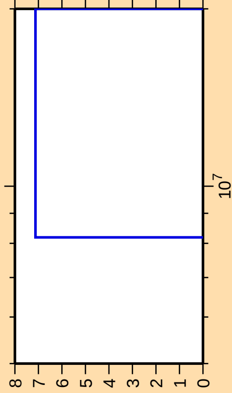
\Delta\sigma/\sigma vs. E for ^{232}\text{Ra}(n,3n\alpha)
