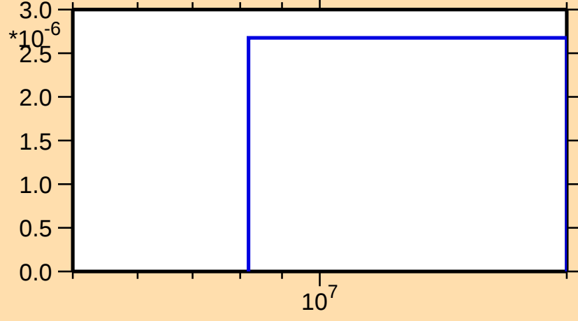
\sigma vs. E for ^{232}\text{Ra}(n,t)
