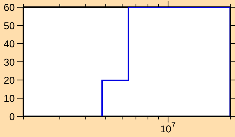
\Delta\sigma/\sigma vs. E for ^{232}\text{Ra}(n,\text{inel.})
