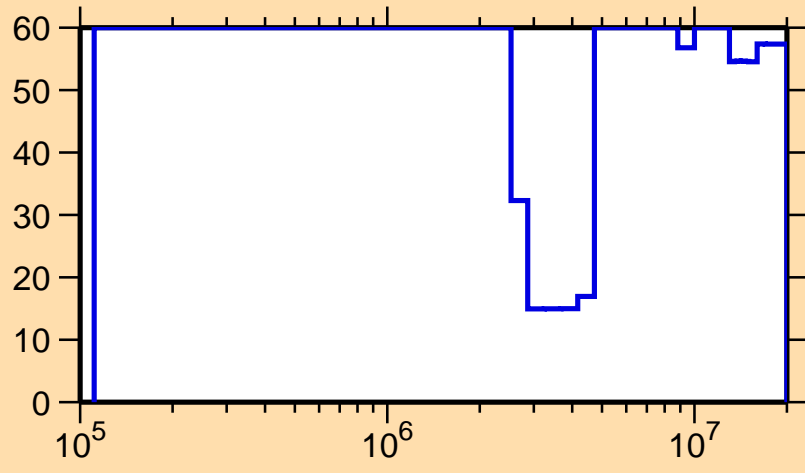
\Delta\sigma/\sigma vs. E for ^{233}\text{Ra}(n,n_1)
