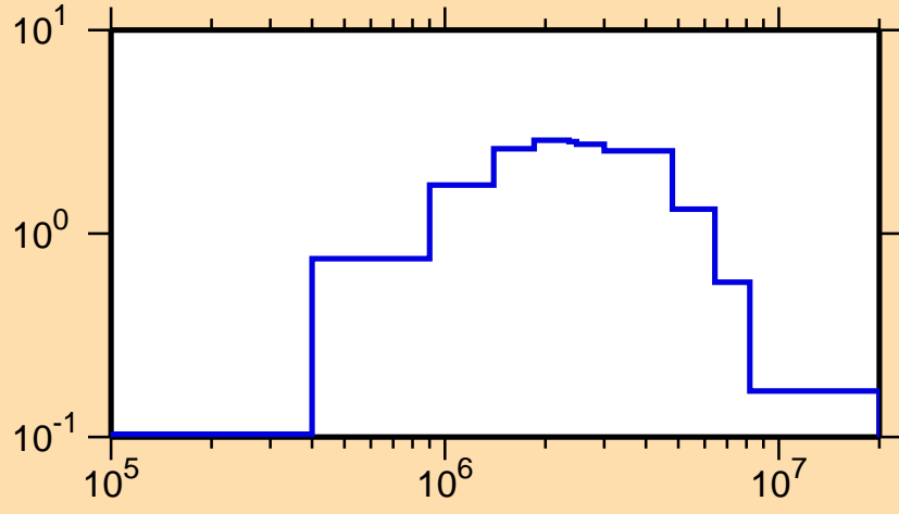
\sigma vs. E for ^{233}\text{Ra}(n,n\text{cont.})
