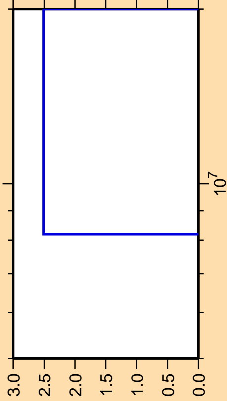
\Delta\sigma/\sigma vs. E for ^{233}\text{Ra}(n,3n\alpha)
