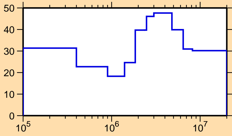
\Delta\sigma/\sigma vs. E for ^{233}\text{Ra}(n,\text{tot.})
