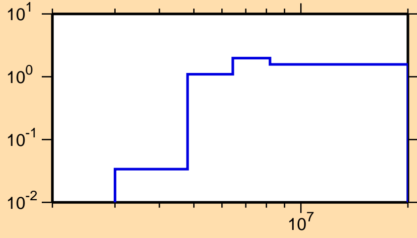
\sigma vs. E for ^{233}\text{Ra}(n,2n)
