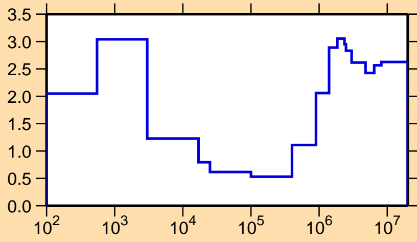
\sigma vs. E for ^{233}\text{Ra}(n,\text{nonel.})
