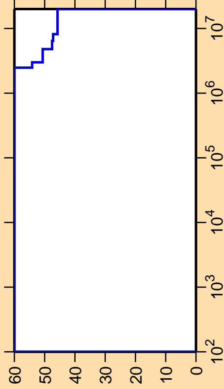
\Delta\sigma/\sigma vs. E for ^{233}\text{Ra}(n,\text{nonel.})
