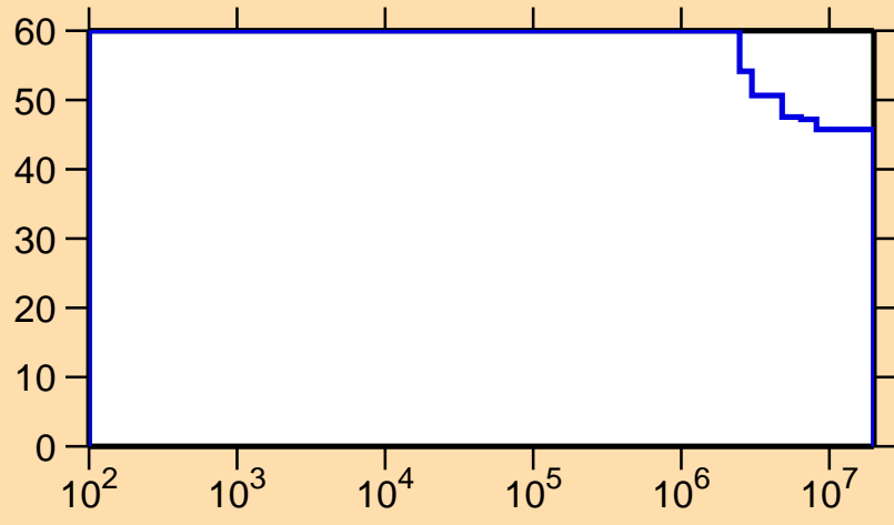
\Delta\sigma/\sigma vs. E for ^{233}\text{Ra}(n,\text{nonel.})
