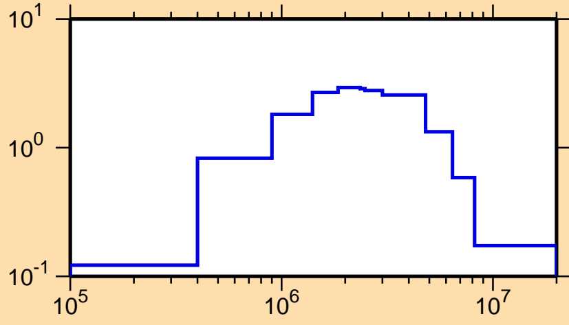
\sigma vs. E for ^{233}\text{Ra}(n,\text{inel.})
