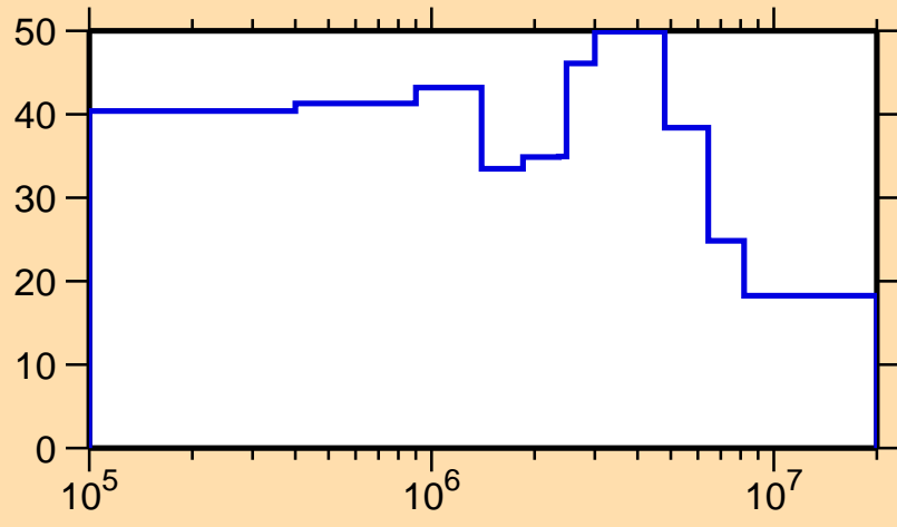
\Delta\sigma/\sigma vs. E for ^{233}\text{Ra}(n,\text{el.})
