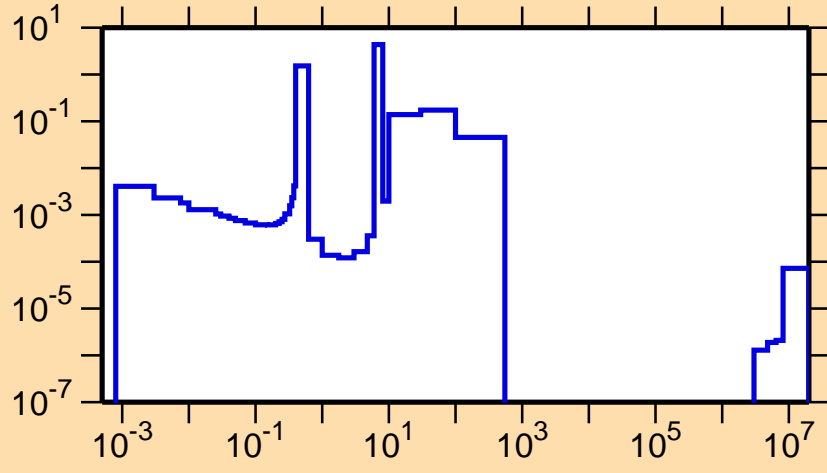
\sigma vs. E for ^{233}\text{Ra}(n,f)
