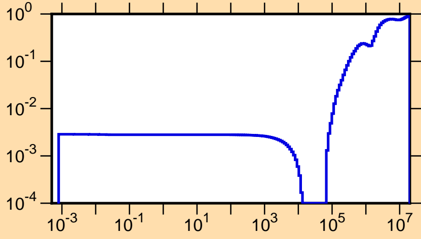
\mu vs. E for ^{234}\text{Ra}(\text{mt251})
