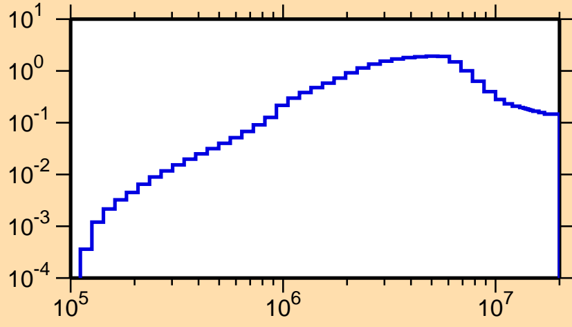
\sigma vs. E for ^{234}\text{Ra}(n,n\text{cont.})
