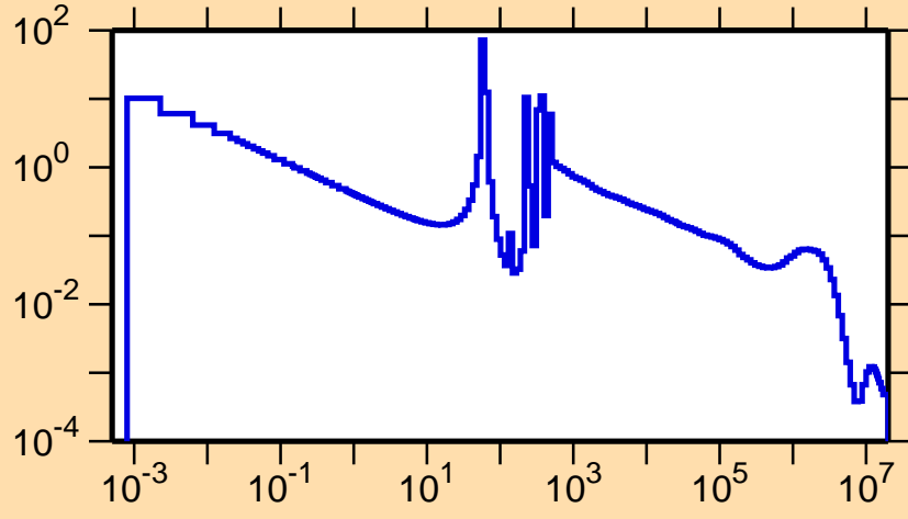
\sigma vs. E for ^{234}\text{Ra}(n,\gamma)
