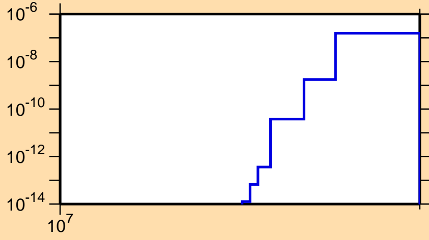
\sigma vs. E for ^{234}\text{Ra}(n,nt)
