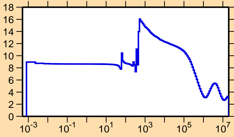
\sigma vs. E for ^{234}\text{Ra}(n,\text{el.})
