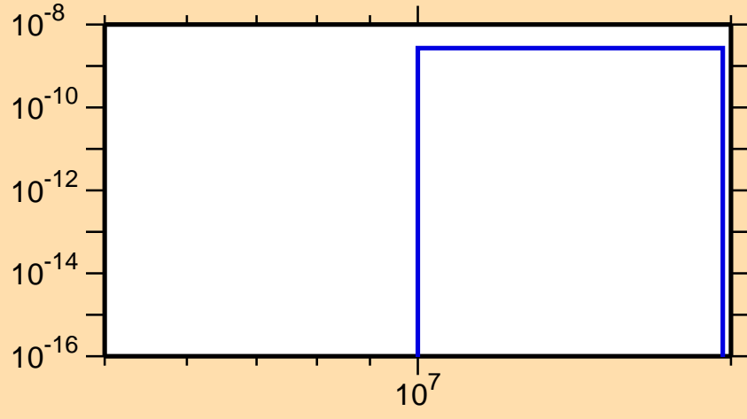
\sigma vs. E for ^{234}\text{Ra}(n,2n\alpha)
