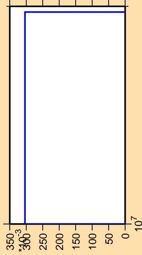
\Delta\sigma/\sigma vs. E for ^{235}\text{Ra}(n,\text{nd})
