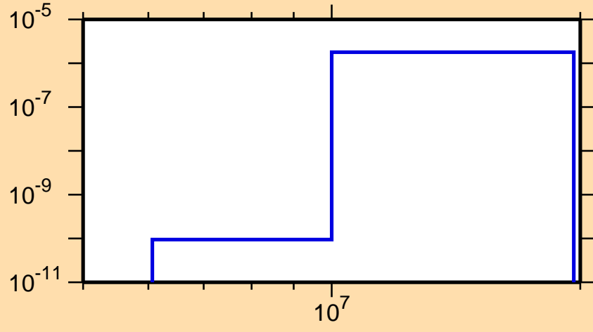
\sigma vs. E for ^{235}\text{Ra}(n,n\alpha)
