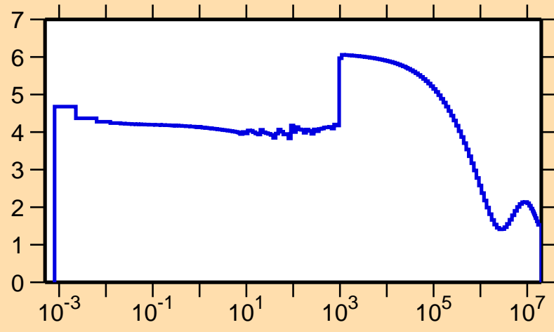
\sigma vs. E for ^{75}\text{Rb}(n,\text{el.})
