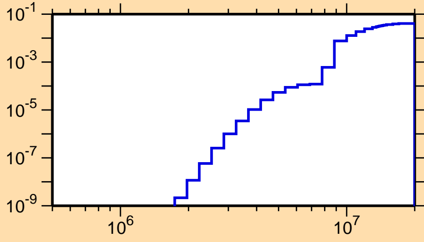
\sigma vs. E for ^{75}\text{Rb}(n,d)
