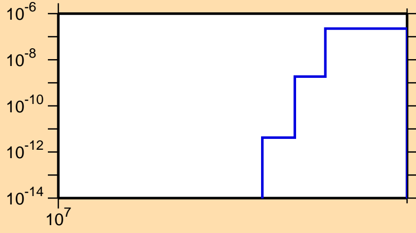
\sigma vs. E for ^{75}\text{Rb}(n,nd)
