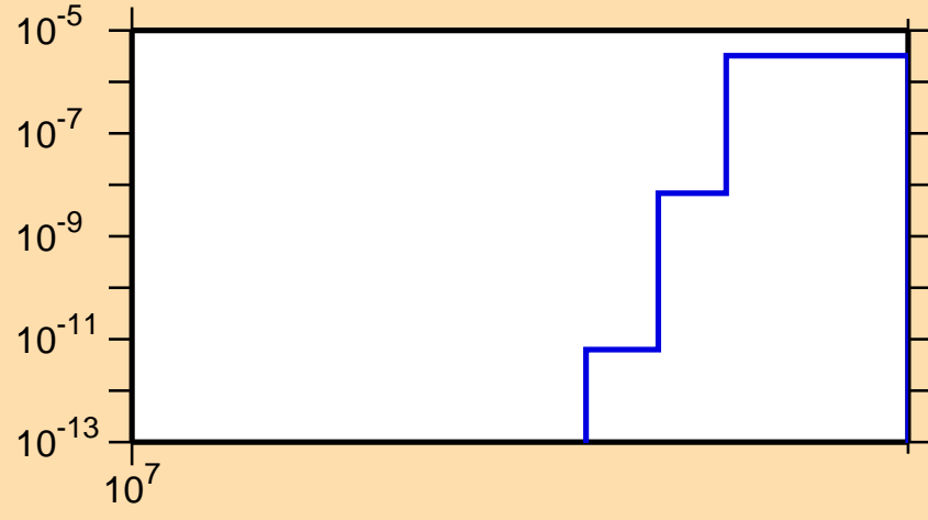
\sigma vs. E for ^{75}\text{Rb}(n,pt)
