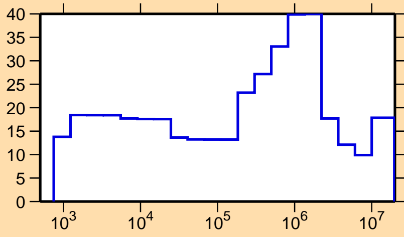
\Delta\sigma/\sigma vs. E for ^{75}\text{Rb}(n,el.)
