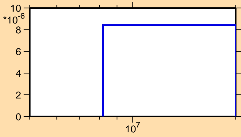
\sigma vs. E for ^{75}\text{Rb} (mt 45)
