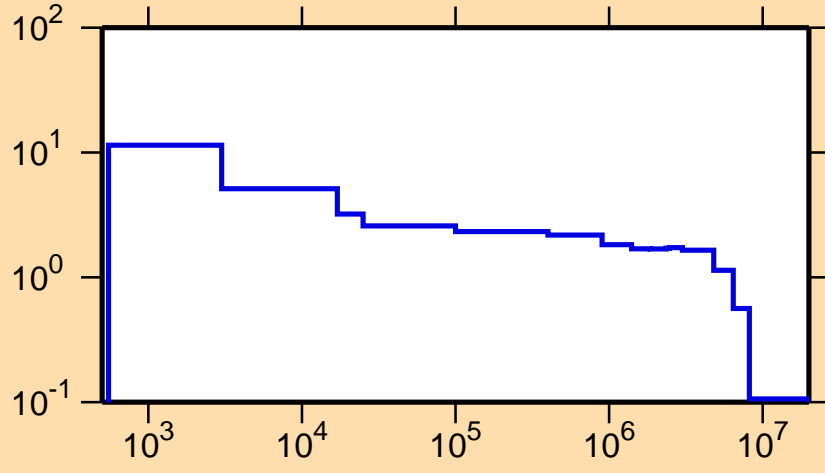
\sigma vs. E for ^{75}\text{Rb}(n,p)
