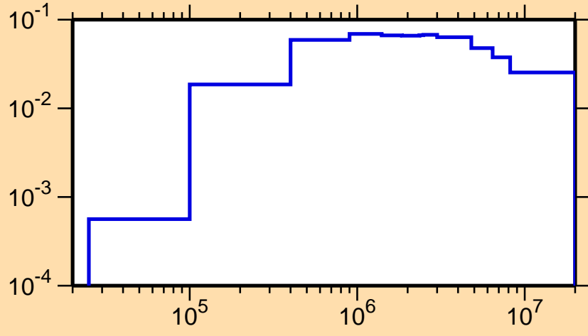
\sigma vs. E for ^{75}\text{Rb}(n,n_1)
