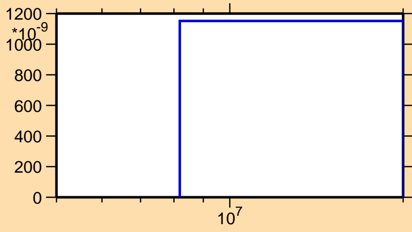
\sigma vs. E for ^{75}\text{Rb}(\text{mt117})
