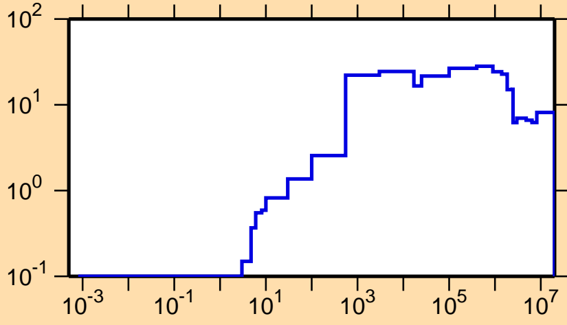
\Delta\sigma/\sigma vs. E for ^{75}\text{Rb}(n,\text{tot.})
