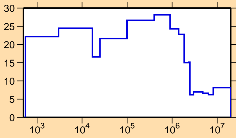
\Delta\sigma/\sigma vs. E for ^{75}\text{Rb}(n,\text{tot.})
