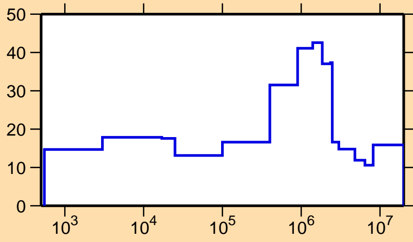
\Delta\sigma/\sigma vs. E for ^{75}\text{Rb}(n,\text{el.})
