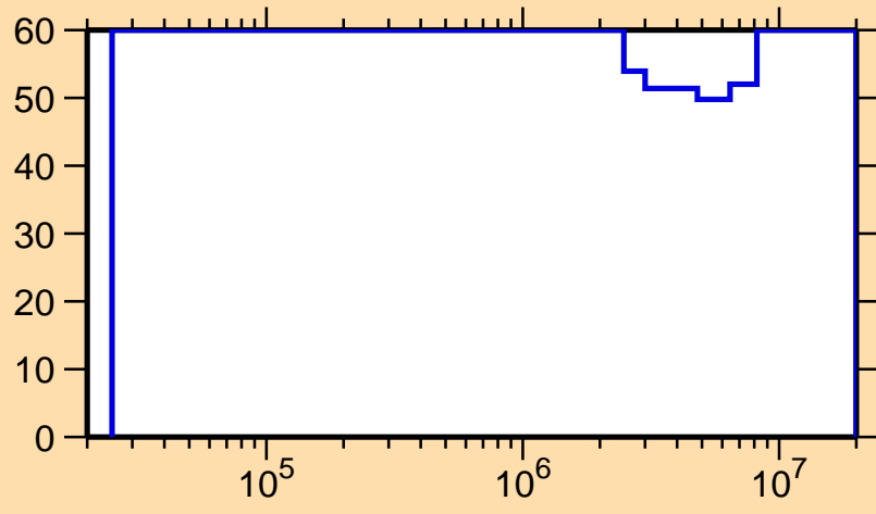
\Delta\sigma/\sigma vs. E for ^{75}\text{Rb}(n,n_1)
