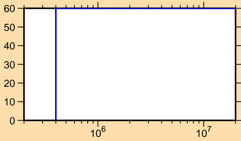
\Delta\sigma/\sigma vs. E for ^{75}\text{Rb}(n,n\text{cont.})
