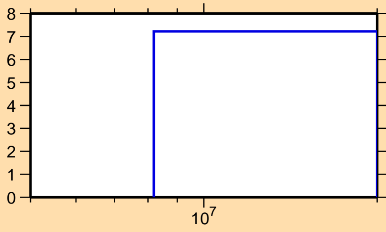
\Delta\sigma/\sigma vs. E for ^{75}\text{Rb}(n,\text{nonel.})
