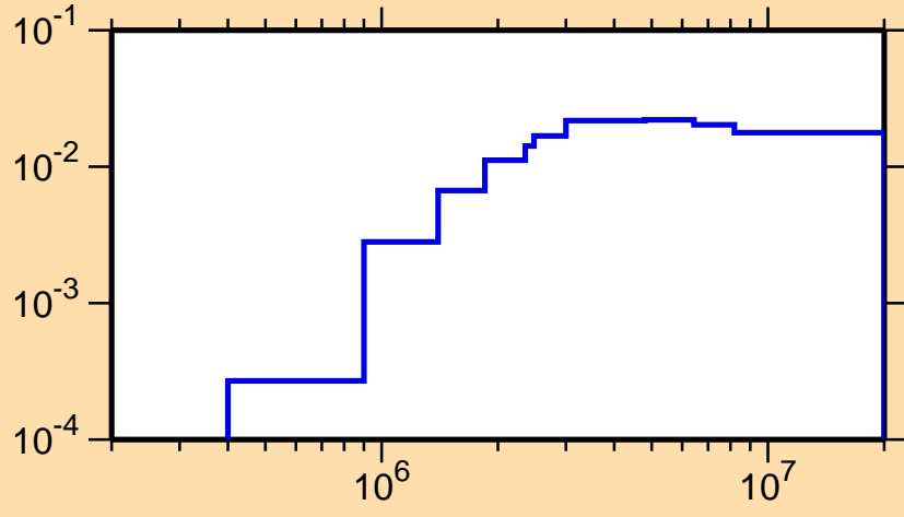
\sigma vs. E for ^{75}\text{Rb}(n,n\text{cont.})
