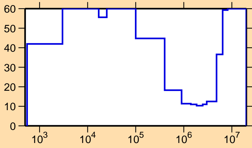
\Delta\sigma/\sigma vs. E for ^{75}\text{Rb}(n,p)
