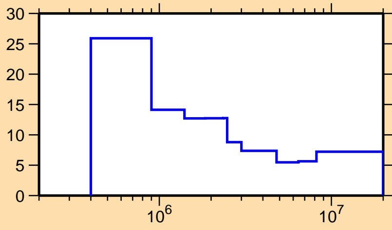
\Delta\sigma/\sigma vs. E for ^{75}\text{Rb}(n,n\text{onel.})
