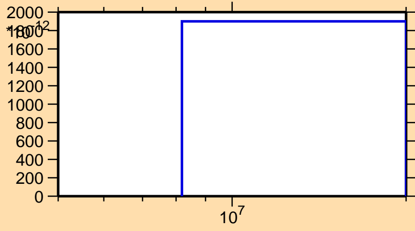
\sigma vs. E for ^{75}\text{Rb}(n,\text{nd})
