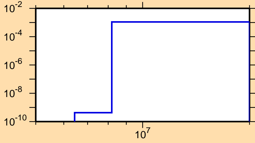
\sigma vs. E for ^{75}\text{Rb}(n,n\alpha)
