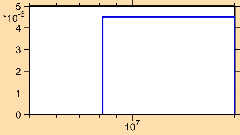
\sigma vs. E for ^{75}\text{Rb}(n,2n)
