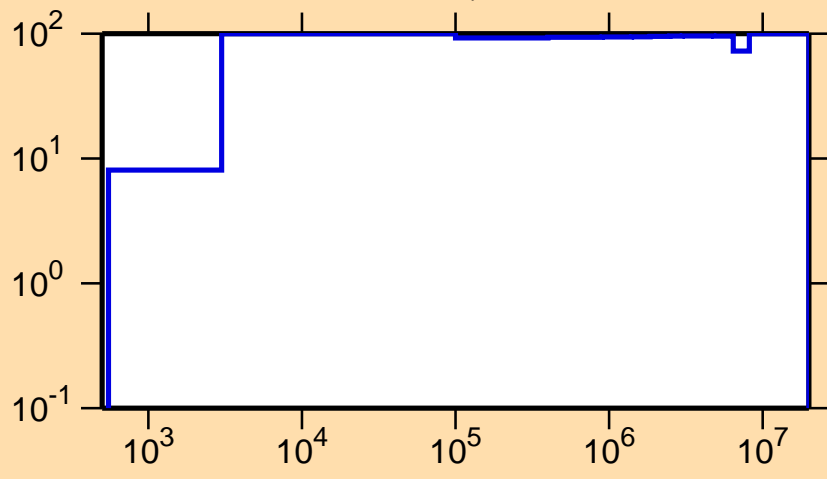
\Delta\sigma/\sigma vs. E for ^{75}\text{Rb}(n,\gamma)
