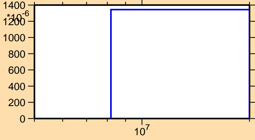
\sigma vs. E for ^{75}\text{Rb}(n,\text{pd})
