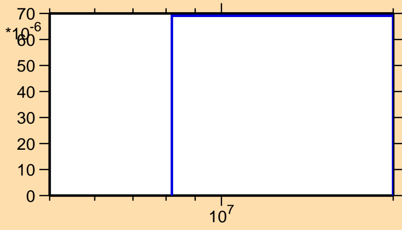
\sigma vs. E for ^{75}\text{Rb}(n,t)
