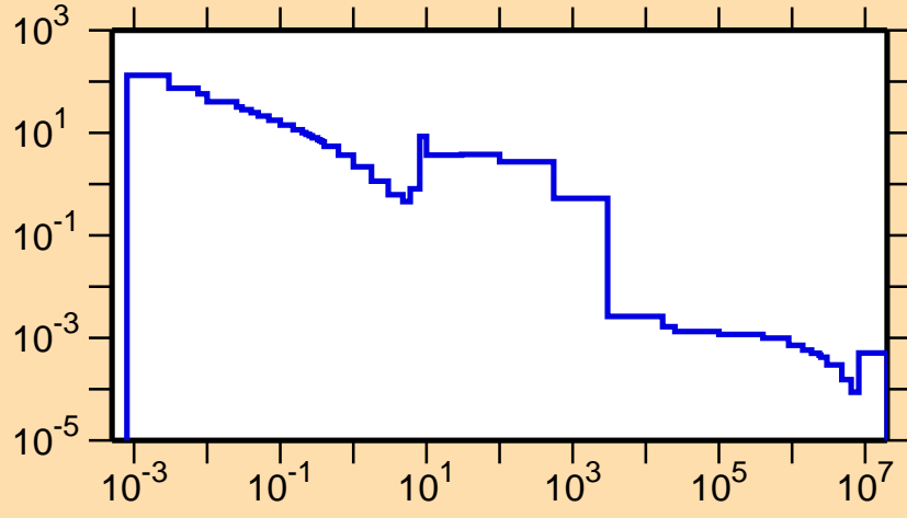
\sigma vs. E for ^{75}\text{Rb}(n,\gamma)
