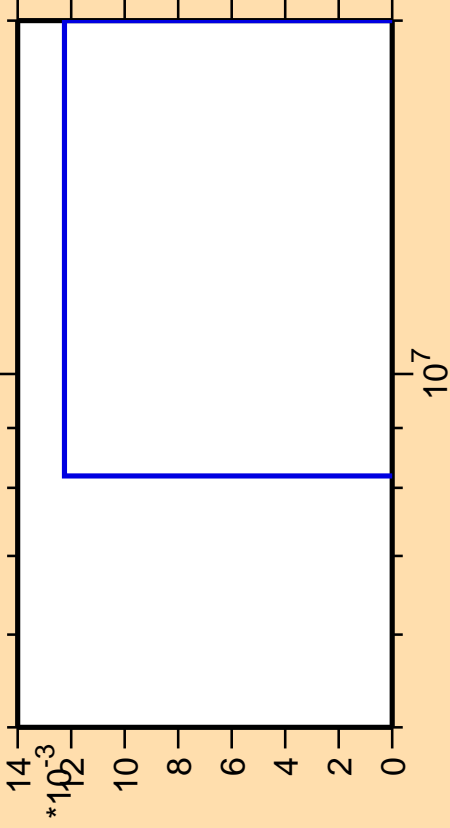
\Delta\sigma/\sigma vs. E for ^{76}\text{Rb}(n,2n\alpha)
