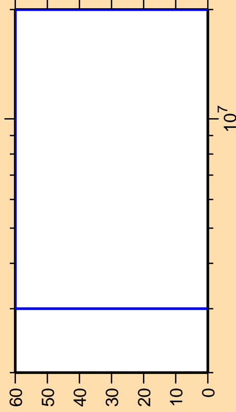
\Delta\sigma/\sigma vs. E for ^{76}\text{Rb}(n,np)
