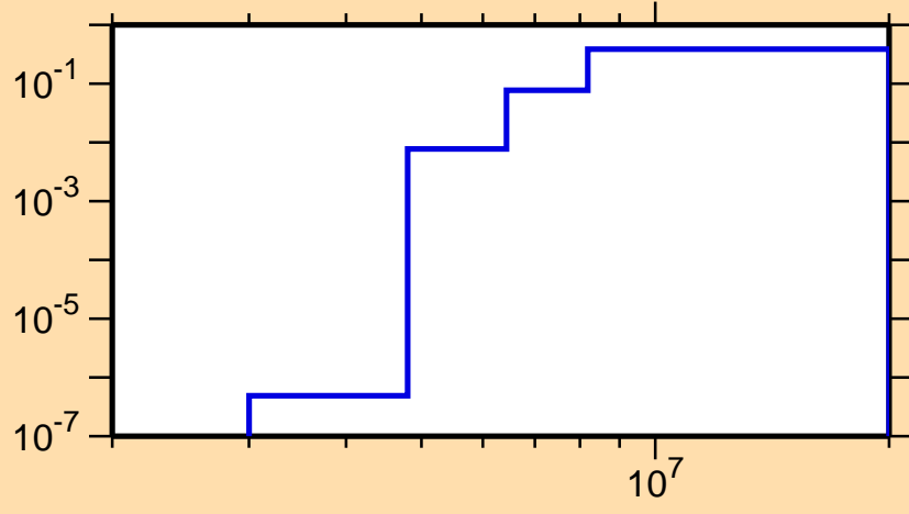
\sigma vs. E for ^{76}\text{Rb}(n,np)
