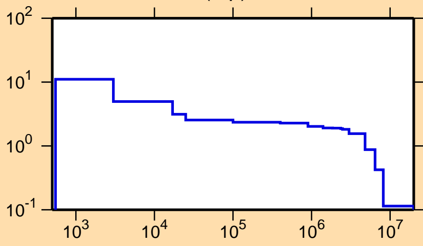
\sigma vs. E for ^{76}\text{Rb}(n,p)
