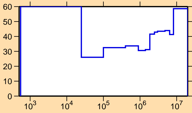
\Delta\sigma/\sigma vs. E for ^{76}\text{Rb}(n,p)
