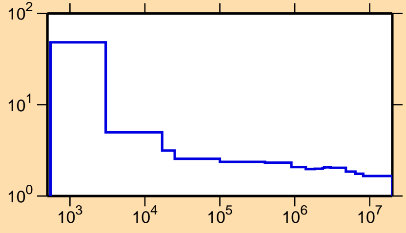
\sigma vs. E for ^{76}\text{Rb}(n,\text{nonel.})
