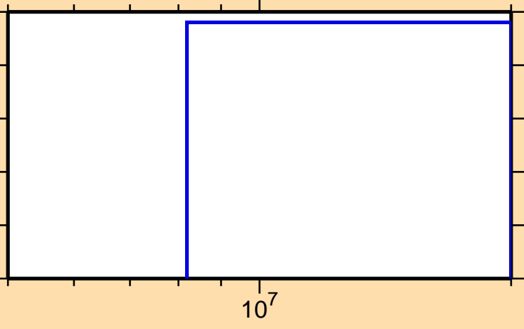
\sigma vs. E for ^{76}\text{Rb}(n,\text{nd})
