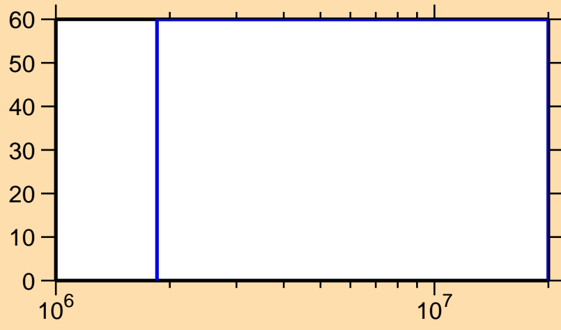
\Delta\sigma/\sigma vs. E for ^{76}\text{Rb}(n,n\text{cont.})
