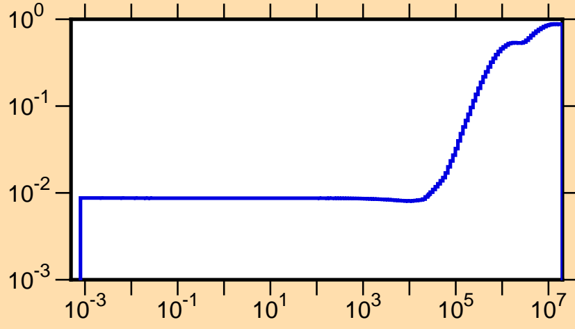
\mu vs. E for ^{77}\text{Rb}(\text{mt251})
