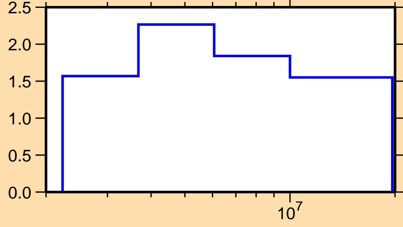
\Delta\sigma/\sigma vs. E for ^{77}\text{Rb}(n,n\text{nonel.})
