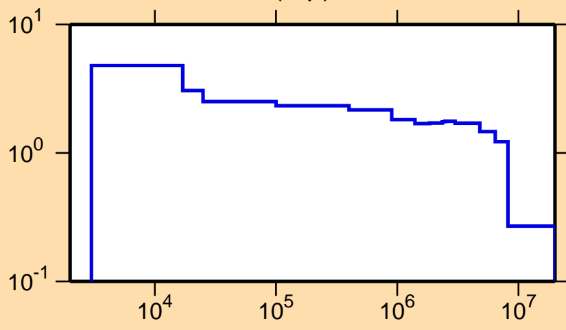
\sigma vs. E for ^{77}\text{Rb}(n,p)
