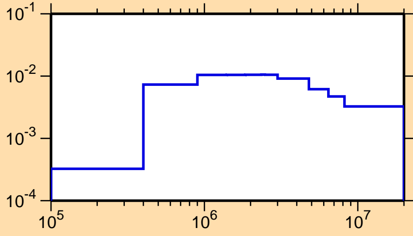
\sigma vs. E for ^{77}\text{Rb}(n,n_3)
