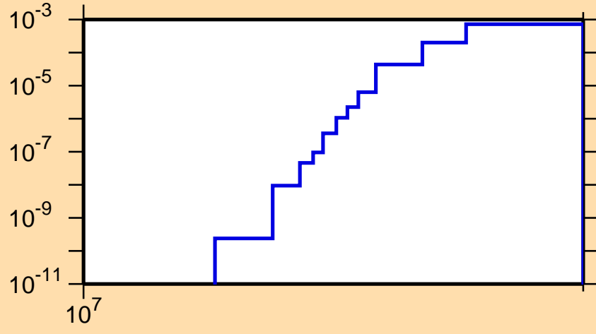
\sigma vs. E for ^{78}\text{Rb}(n,nd)
