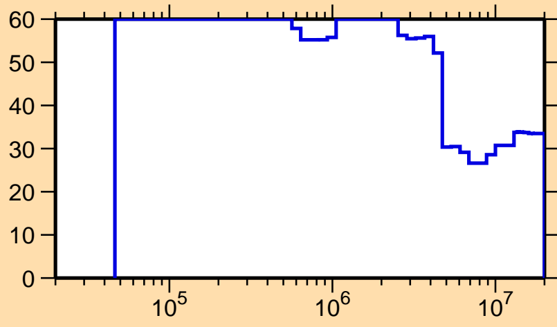
\Delta\sigma/\sigma vs. E for ^{78}\text{Rb}(n,n_1)
