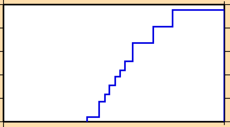
\sigma vs. E for ^{78}\text{Rb}(\text{mt117})
