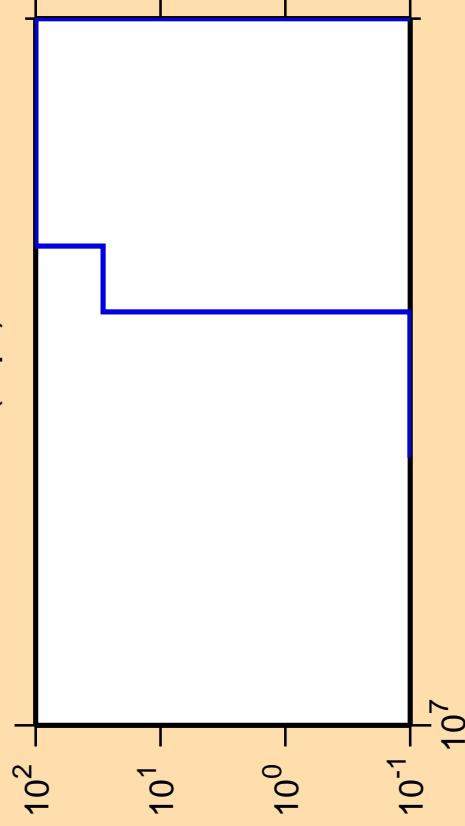
\Delta\sigma/\sigma vs. E for ^{78}\text{Rb}(n,pt)
