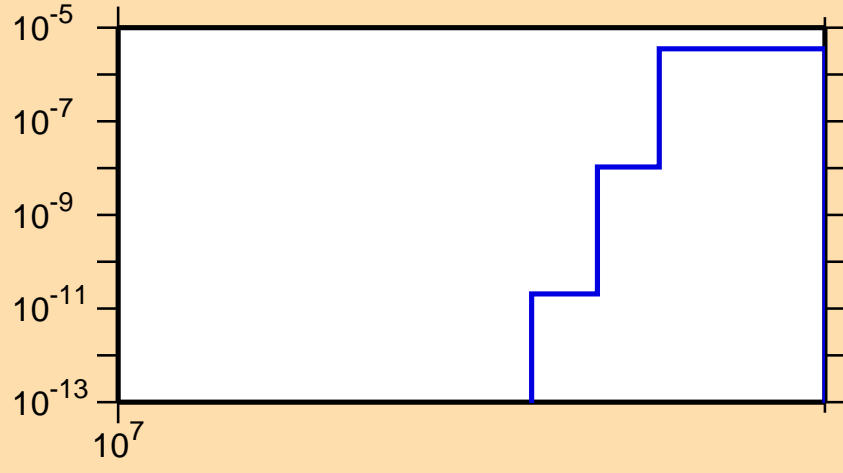
\sigma vs. E for ^{78}\text{Rb}(n,pt)
