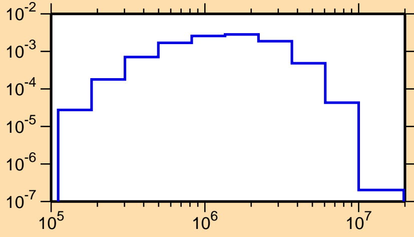
\sigma vs. E for ^{78}\text{Rb}(n,n_3)
