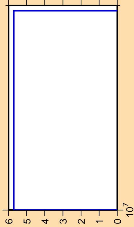
\Delta\sigma/\sigma vs. E for ^{78}\text{Rb}(n,2n\alpha)
