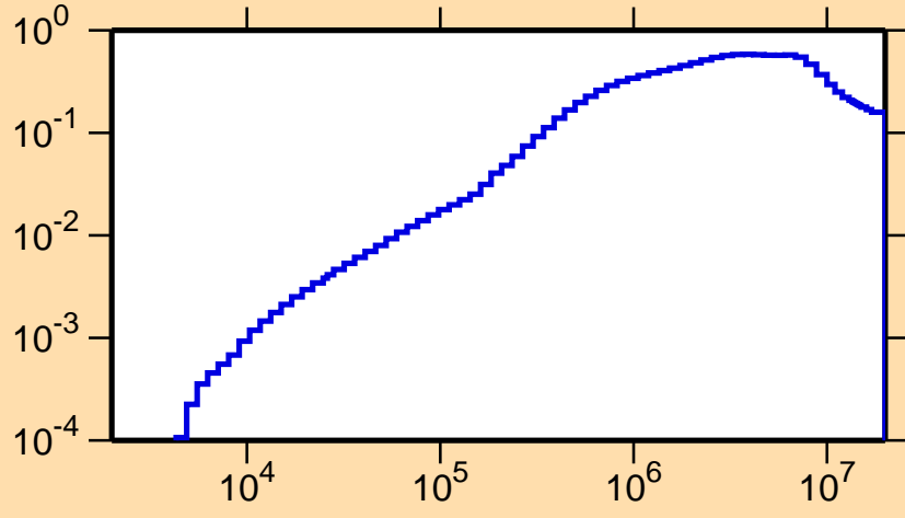
\sigma vs. E for ^{78}\text{Rb}(n,\text{inel.})
