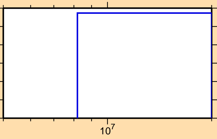
\sigma vs. E for ^{78}\text{Rb}(n,nd)
