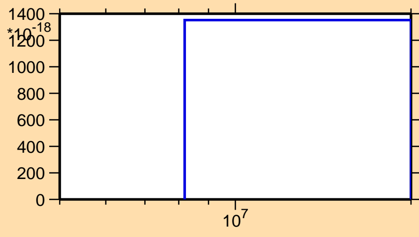
\sigma vs. E for ^{78}\text{Rb}(n,nt)
