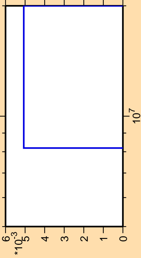
\Delta\sigma/\sigma vs. E for ^{78}\text{Rb}(n,nt)
