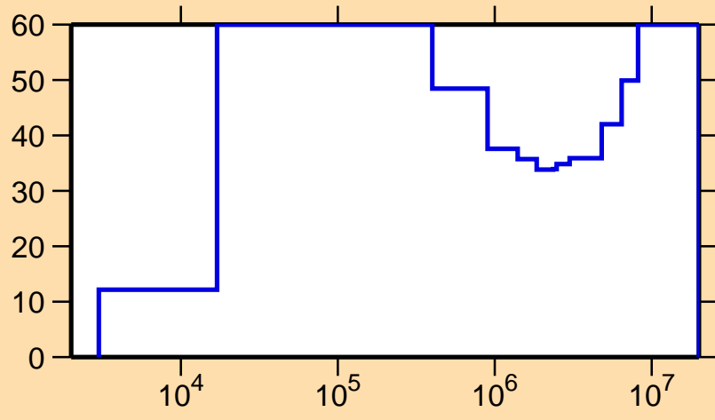
\Delta\sigma/\sigma vs. E for ^{78}\text{Rb}(n,\gamma)
