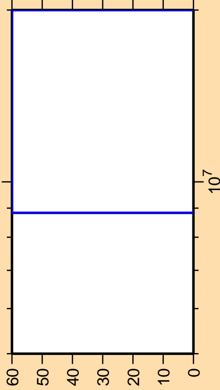
\Delta\sigma/\sigma vs. E for ^{79}\text{Rb}(n,t)
