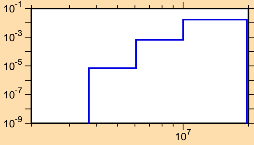
\sigma vs. E for ^{79}\text{Rb}(n,d)
