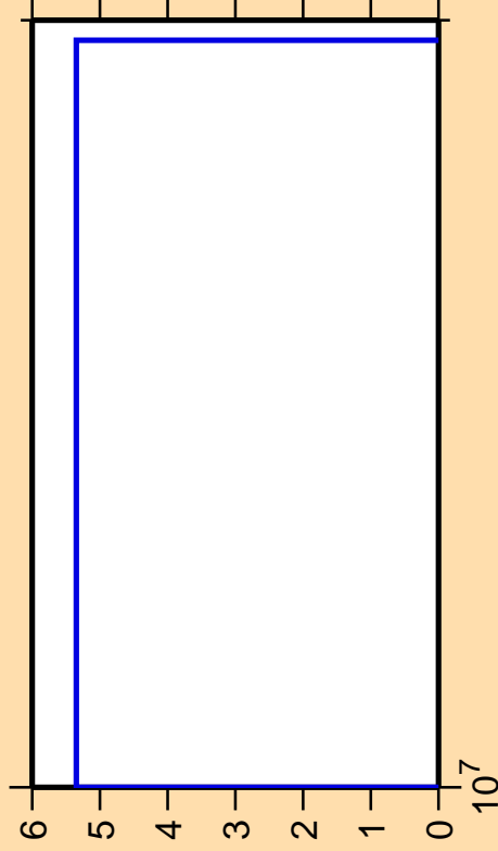
\Delta\sigma/\sigma vs. E for ^{79}\text{Rb}(n,nt)
