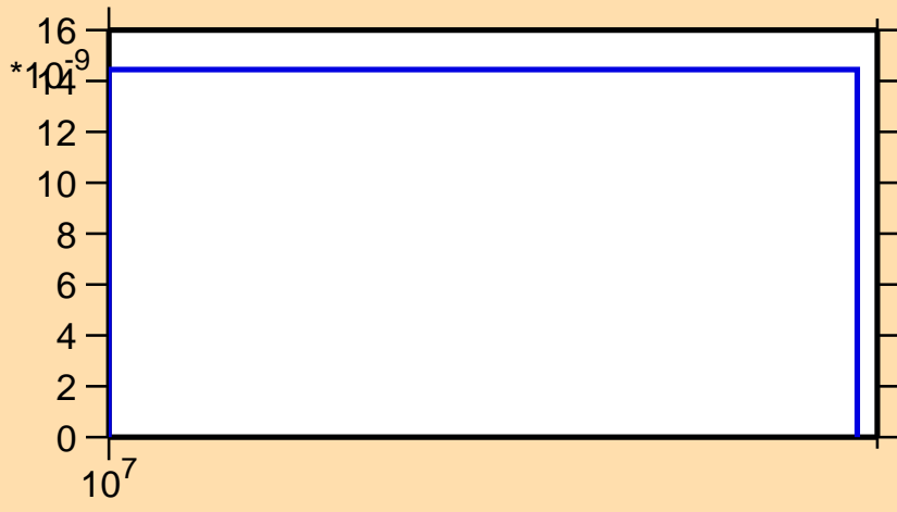
\sigma vs. E for ^{79}\text{Rb} (mt117)
