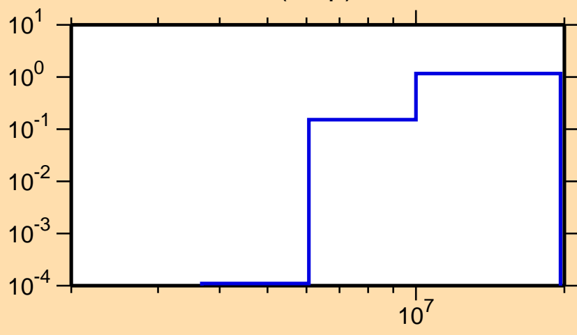
\sigma vs. E for ^{79}\text{Rb}(n,np)
