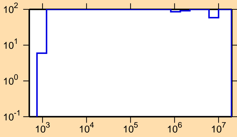
\Delta\sigma/\sigma vs. E for ^{79}\text{Rb}(n,\gamma)
