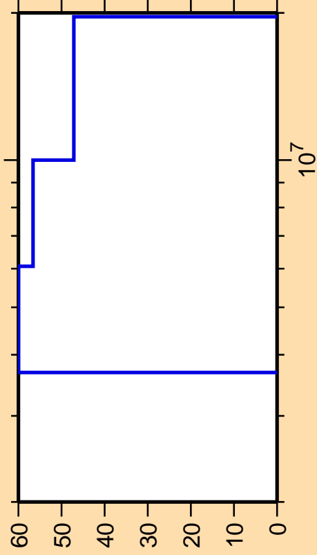
\Delta\sigma/\sigma vs. E for ^{79}\text{Rb}(n,np)
