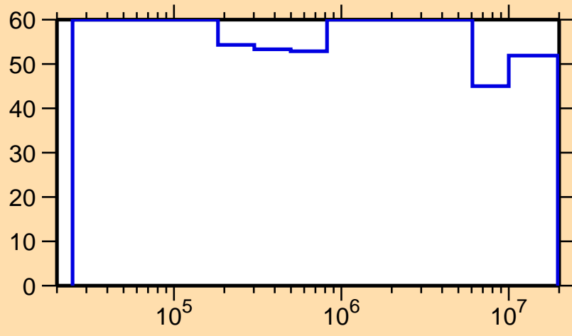
\Delta\sigma/\sigma vs. E for ^{79}\text{Rb}(n,n_1)
