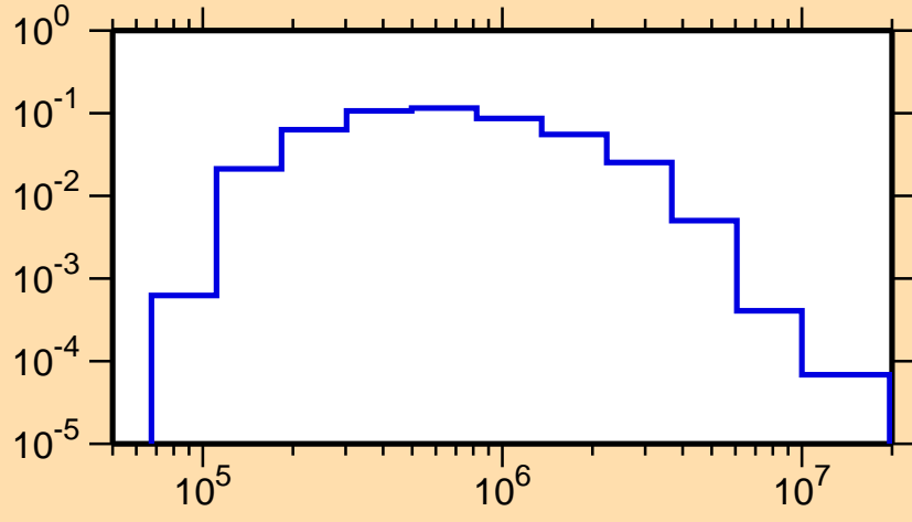
\sigma vs. E for ^{79}\text{Rb}(n,n_2)
