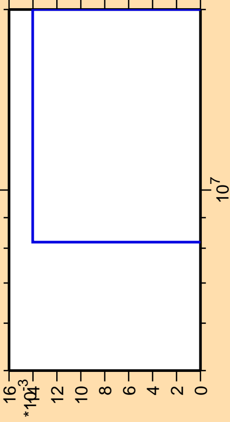
\Delta\sigma/\sigma vs. E for ^{79}\text{Rb} (mt 34)
