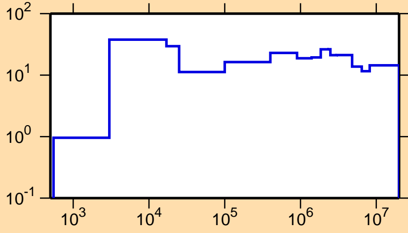
\Delta\sigma/\sigma vs. E for ^{79}\text{Rb}(n,\text{el.})
