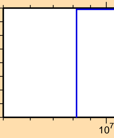
\sigma vs. E for ^{79}\text{Rb}(n,\text{He}3)
