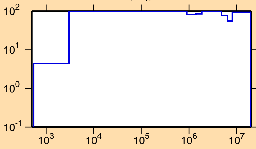
\Delta\sigma/\sigma vs. E for ^{79}\text{Rb}(n,\gamma)
