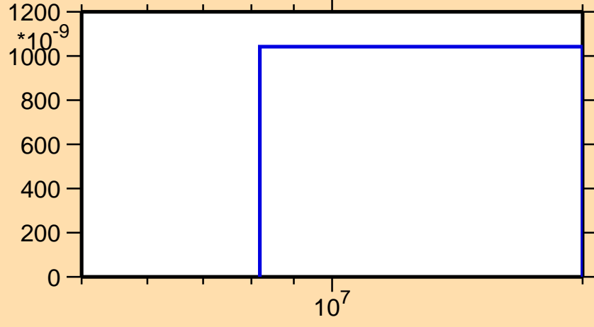
\sigma vs. E for ^{79}\text{Rb}(n,2np)
