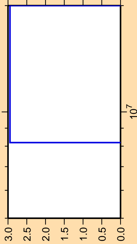
\Delta\sigma/\sigma vs. E for ^{79}\text{Rb}(n,\text{pt})
