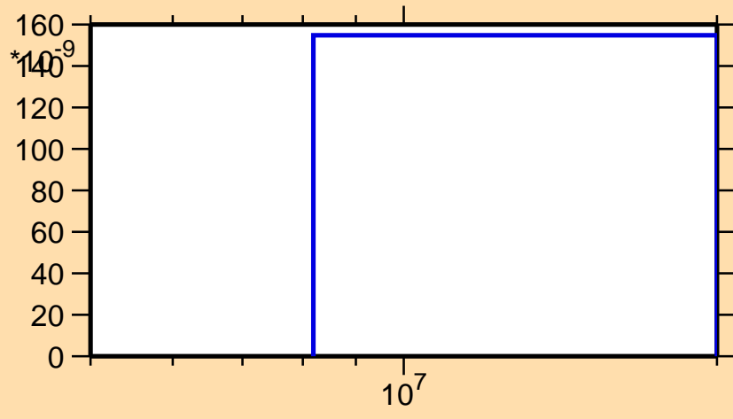
\sigma vs. E for ^{79}\text{Rb}(n,\text{nd})
