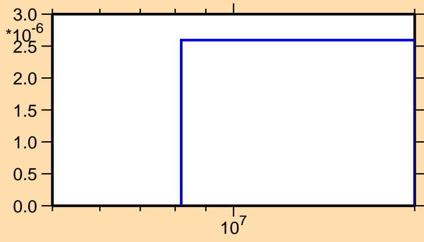
\sigma vs. E for ^{79}\text{Rb}(n,\text{pd})
