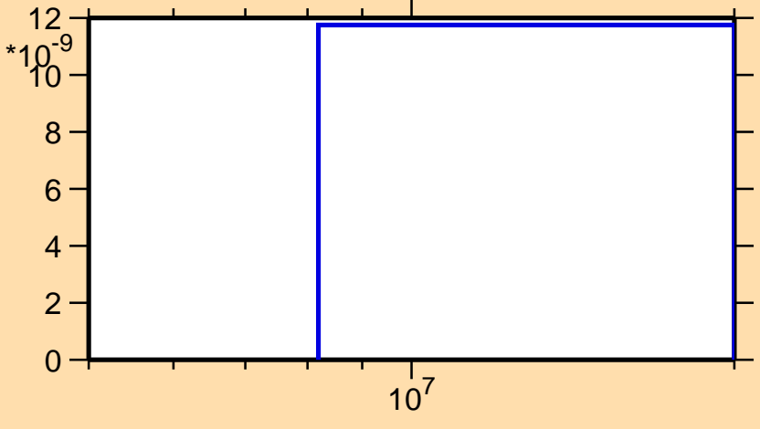
\sigma vs. E for ^{79}\text{Rb}(\text{mt117})
