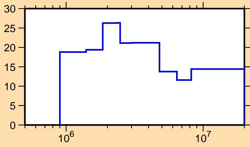
\Delta\sigma/\sigma vs. E for ^{79}\text{Rb}(n,\text{el.})
