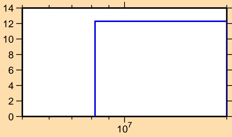
\Delta\sigma/\sigma vs. E for ^{79}\text{Rb}(n,\text{nonel.})
