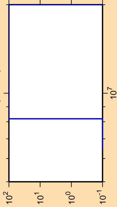
\Delta\sigma/\sigma vs. E for ^{79}\text{Rb}(n,\text{He}3)
