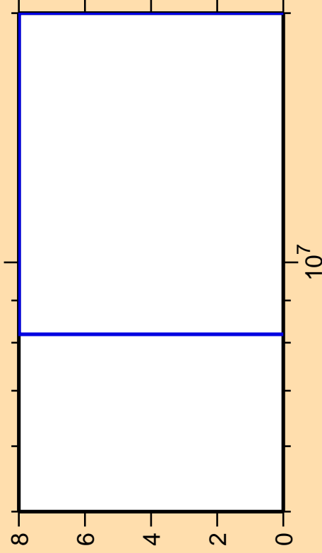
\Delta\sigma/\sigma vs. E for ^{79}\text{Rb}(n,nt)
