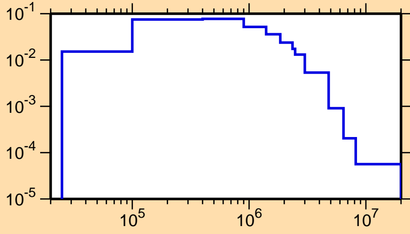
\sigma vs. E for ^{79}\text{Rb}(n,n_1)
