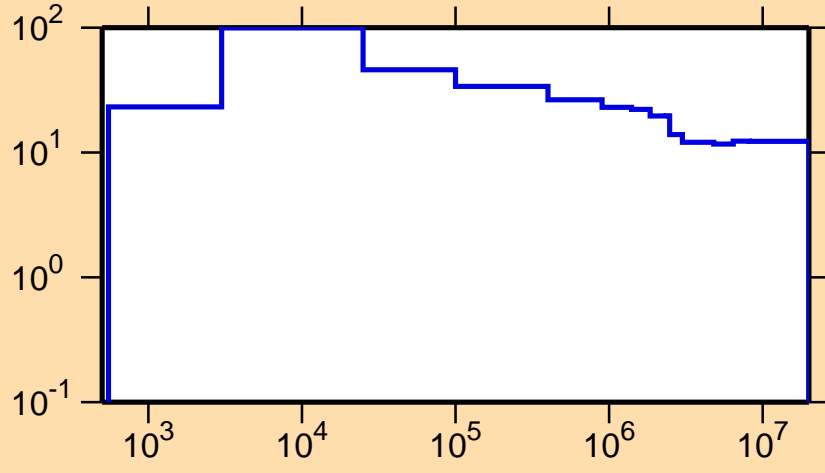
\Delta\sigma/\sigma vs. E for ^{79}\text{Rb}(n,\text{nonel.})
