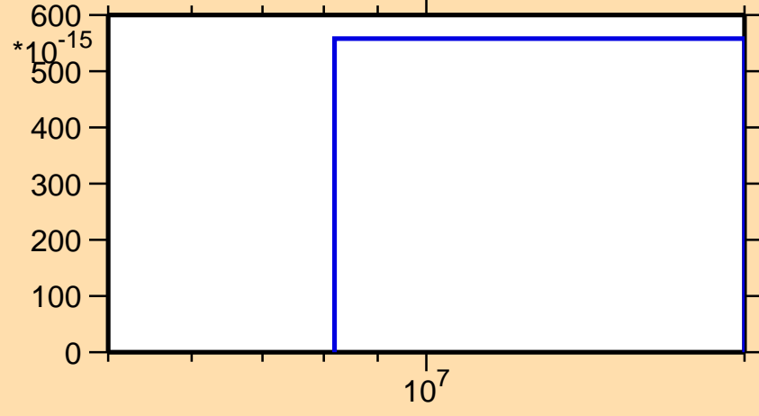
\sigma vs. E for ^{79}\text{Rb}(n,\text{pt})
