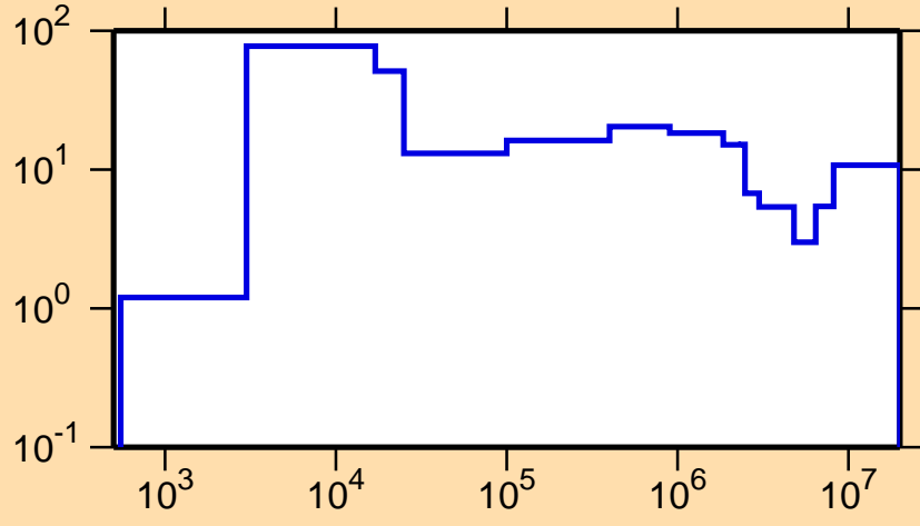
\Delta\sigma/\sigma vs. E for ^{79}\text{Rb}(n,\text{tot.})
