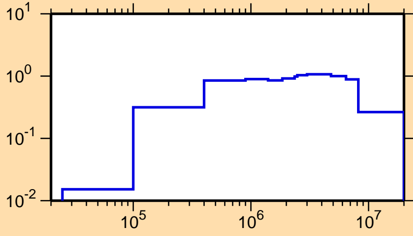
\sigma vs. E for ^{79}\text{Rb}(n,\text{inel.})
