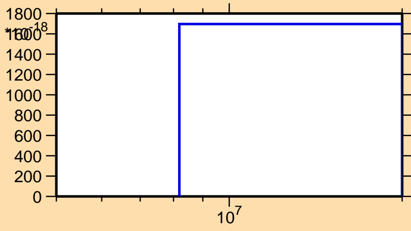
\sigma vs. E for ^{79}\text{Rb} (mt 34)
