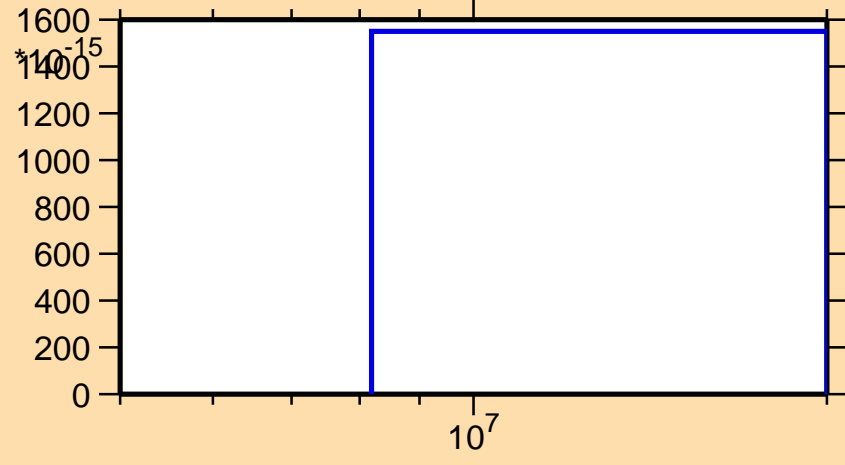
\sigma vs. E for ^{79}\text{Rb}(n,nt)
