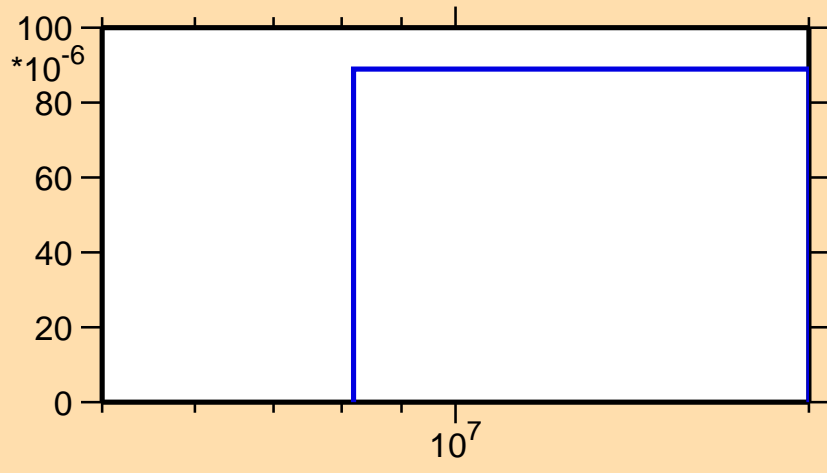
\sigma vs. E for ^{79}\text{Rb}(n,t)
