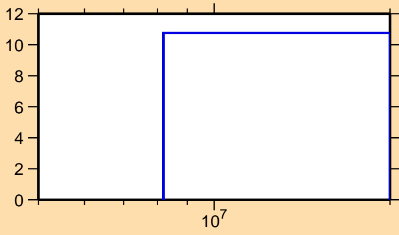
\Delta\sigma/\sigma vs. E for ^{79}\text{Rb}(n,\text{tot.})
