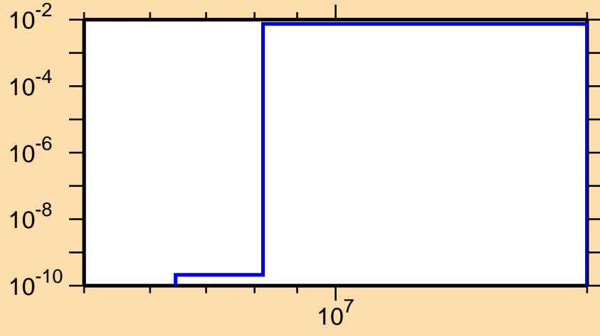
\sigma vs. E for ^{79}\text{Rb}(n,n\alpha)
