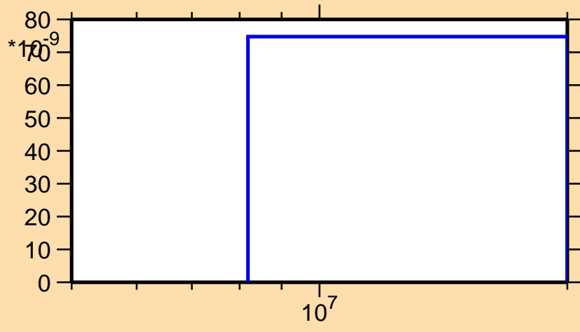
\sigma vs. E for ^{79}\text{Rb} (mt 45)
