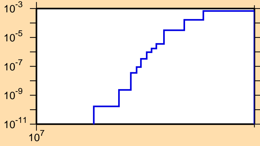
\sigma vs. E for ^{80}\text{Rb}(n,nd)
