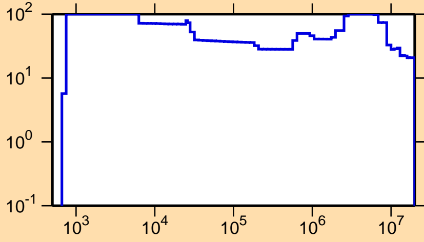
\Delta\sigma/\sigma vs. E for ^{80}\text{Rb}(n,p)
