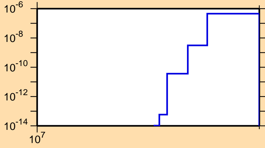
\sigma vs. E for ^{80}\text{Rb} (mt 45)
