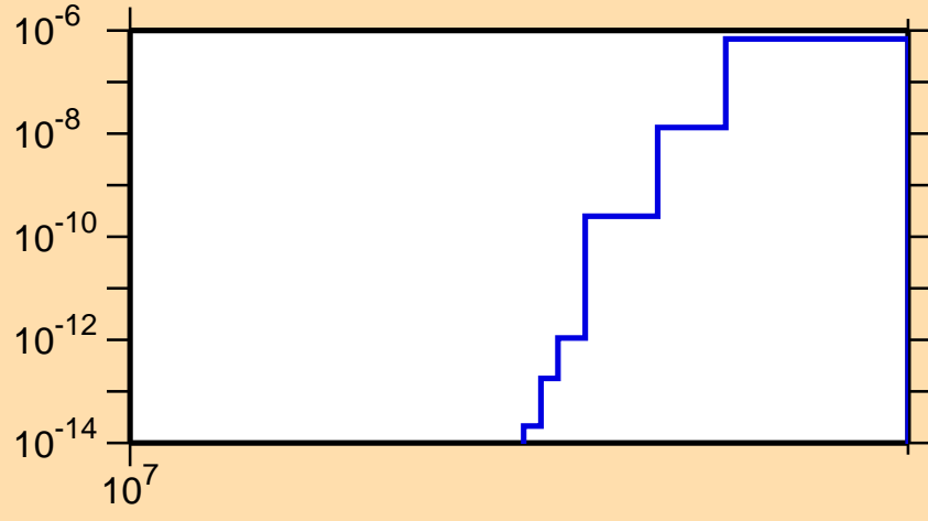
\sigma vs. E for ^{80}\text{Rb}(n,\text{pd})
