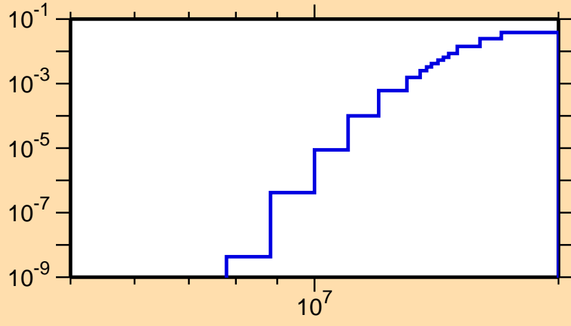
\sigma vs. E for ^{80}\text{Rb}(n,n\alpha)
