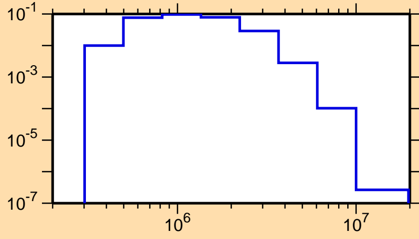
\sigma vs. E for ^{80}\text{Rb}(n,n_4)
