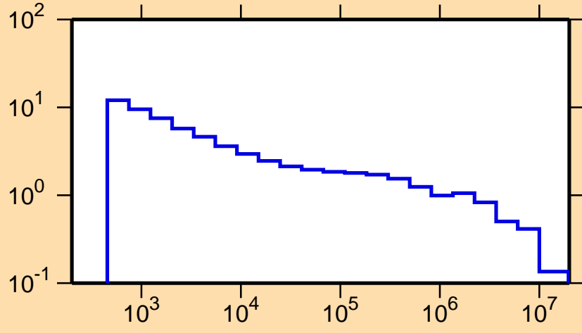
\sigma vs. E for ^{80}\text{Rb}(n,p)
