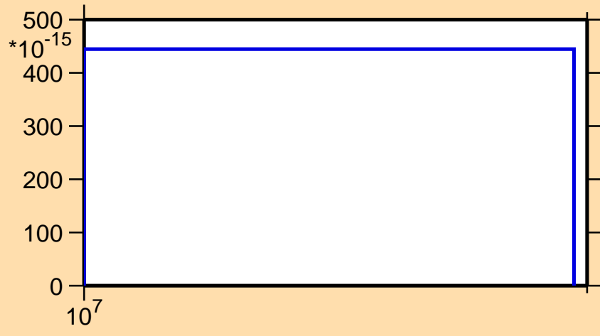
\sigma vs. E for ^{80}\text{Rb}(n,nt)
