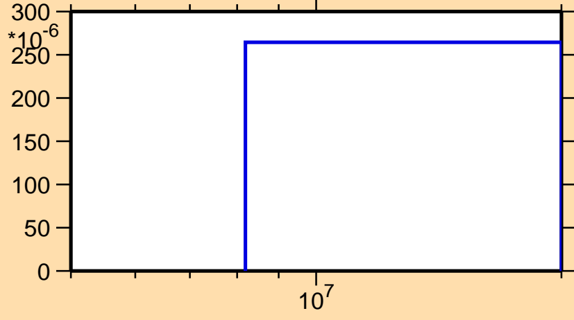
\sigma vs. E for ^{80}\text{Rb}(n,2np)
