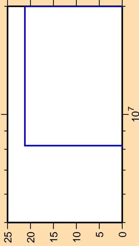
\Delta\sigma/\sigma vs. E for ^{80}\text{Rb} (mt 34)
