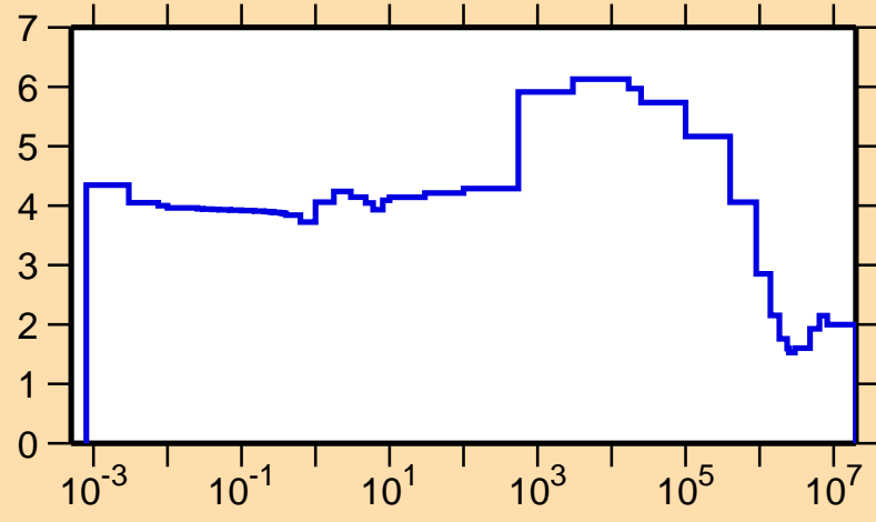
\sigma vs. E for ^{80}\text{Rb}(n,\text{el.})
