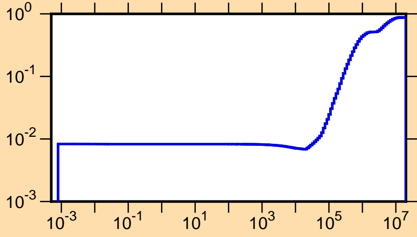
\mu vs. E for ^{81}\text{Rb}(\text{mt251})
