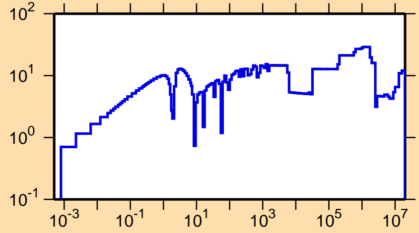
\Delta\sigma/\sigma vs. E for ^{81}\text{Rb}(n,\text{tot.})
