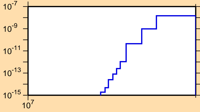
\sigma vs. E for ^{81}\text{Rb}(\text{mt117})
