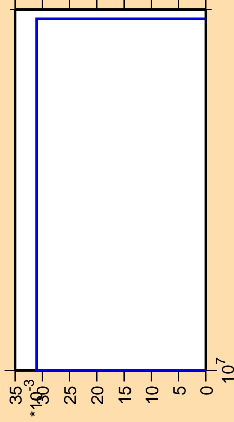
\Delta\sigma/\sigma vs. E for ^{81}\text{Rb}(n,2n\alpha)
