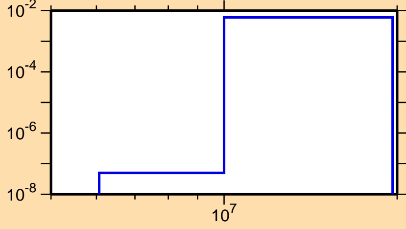
\sigma vs. E for ^{81}\text{Rb}(n,n\alpha)
