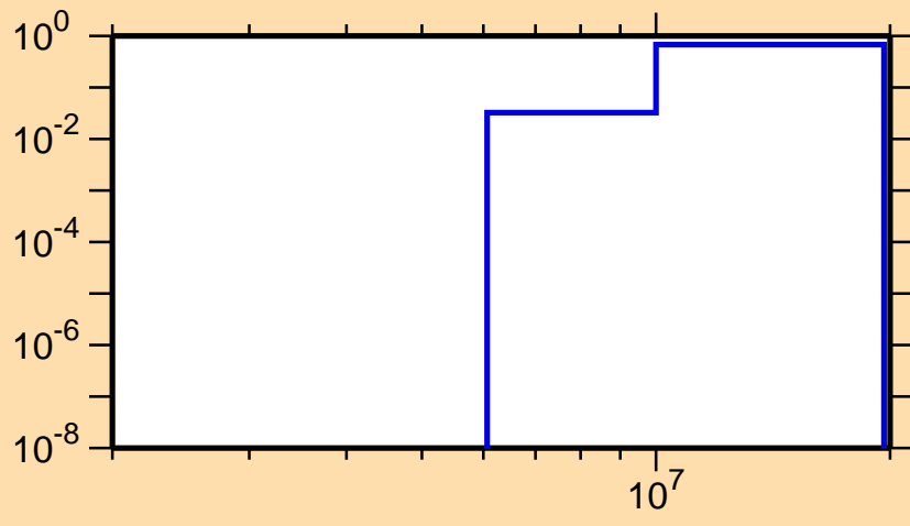
\sigma vs. E for ^{81}\text{Rb}(n,np)
