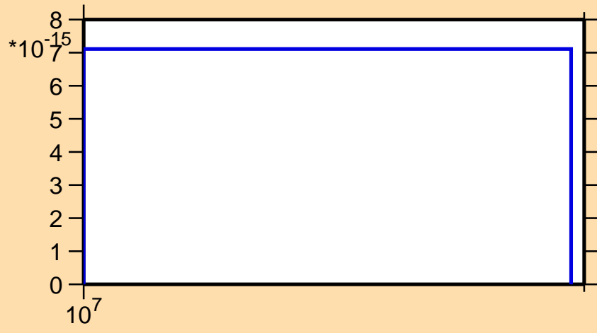
\sigma vs. E for ^{81}\text{Rb}(n,2n\alpha)
