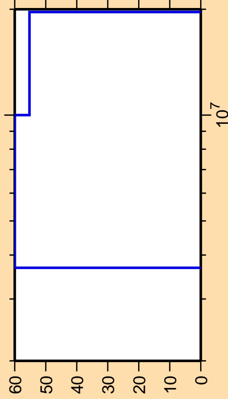
\Delta\sigma/\sigma vs. E for ^{81}\text{Rb}(n,np)
