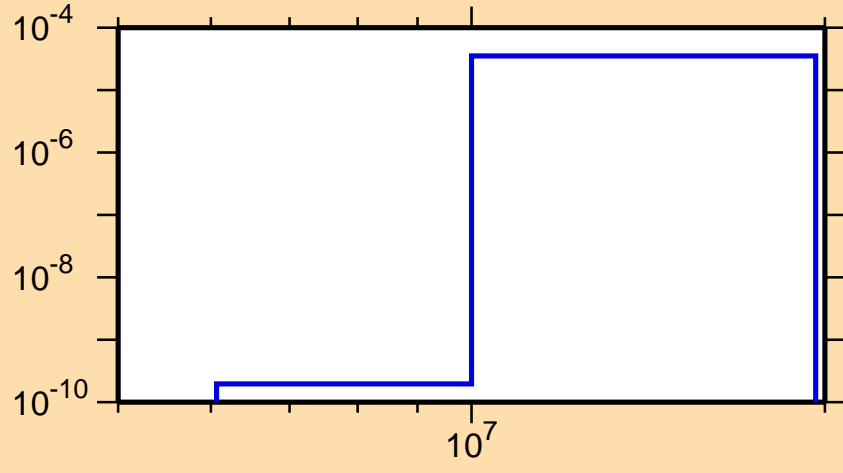
\sigma vs. E for ^{81}\text{Rb}(n,p\alpha)
