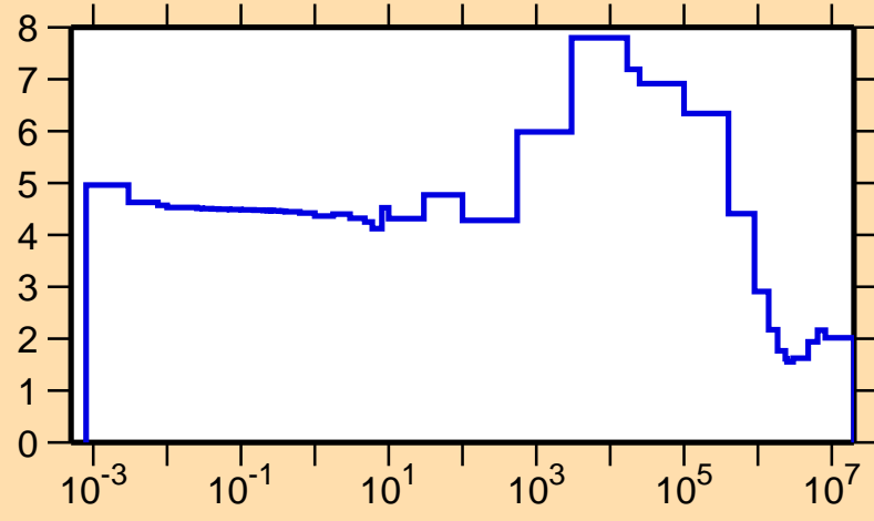
\sigma vs. E for ^{81}\text{Rb}(n,\text{el.})
