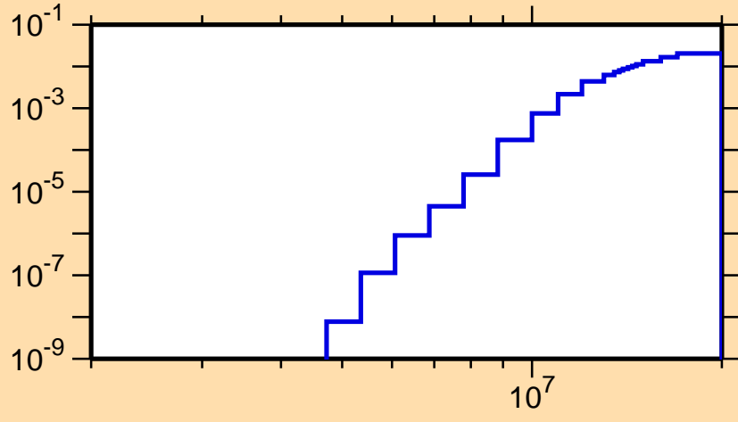
\sigma vs. E for ^{81}\text{Rb}(n,d)
