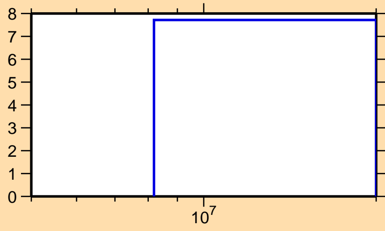
\Delta\sigma/\sigma vs. E for ^{81}\text{Rb}(n,\text{tot.})
